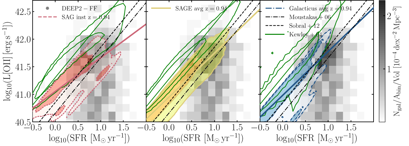
Figure 11. Intrinsic [O II] luminosity as a function of the SFR from the MultiDark-Galaxies at z \sim 1 (salmon, yellow and blue, filled contours), compared with the DEEP2-FF observations at 0.9 < z < 1.1 (grey, shaded squares, colour coded with the density of emitters per 2D bin area). The innermost (outermost) contour represents 68 per cent (95 per cent) of the galaxy distributions. For SAG model galaxies, the [O II] luminosities have been computed from instantaneous SFRs, while for the other SAMs they are based on average SFRs. Both data and model ELGs are selected imposing a minimum [O II] flux of 5 \times 10^{-18} erg s^{-1} cm^{-2} . The thick, coloured, diagonal lines are the linear fits to each SAM distribution, and their best-fitting parameters are reported in Table 2. The black dot-dashed and dashed, diagonal lines are the L[O II] predictions obtained from the SFR range of interest using equations (15) and (16), respectively. The green, empty contours are the Kewley et al. (2004) predictions obtained using equation (17) with SFR and cold gas metallicity as inputs. The green, solid lines are the same predictions assuming median metallicity values in bins of SFR.
