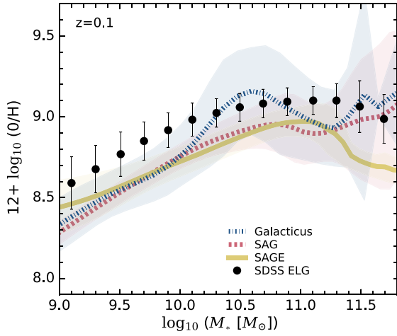
Figure 10. Mean gas-phase oxygen abundance in bins of stellar mass of the SDSS emission line galaxies at z \sim 0.1 (Favole et al. 2017) compared to the MultiDark-Galaxies models. The abundance is computed for the SAMs using equation (18). The error bars on the SDSS measurements are the 1\sigma scatter around the mean.
