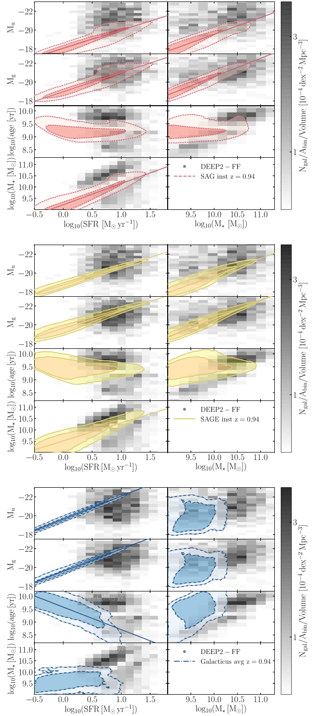
Figure C1. Comparison of pairs of properties for MULTIDARK-GALAXIES at z = 1 (contours) and DEEP2-FF observations at 0.9 < z < 1.1 (grey, shaded squares). The colour bars show the number density of DEEP2 galaxies in each square. From top to bottom, we display SAG, SAGE, and GALACTICUS results. A minimum [\text{O II}] flux cut of 5 \times 10^{-18} \text{ erg s}^{-1} \text{ cm}^{-2} has been applied to both data and model galaxies. In each set of panels, from top to bottom, we compare broad-band u and g absolute magnitudes, age and stellar mass as a function of, from left to right, average SFR and stellar mass. The model contours, from inner to outer, represent 68 percent and 95 percent of the distributions. The diagonal lines are the linear fits showing the significant correlations, whose coefficients are given in Table 2.
