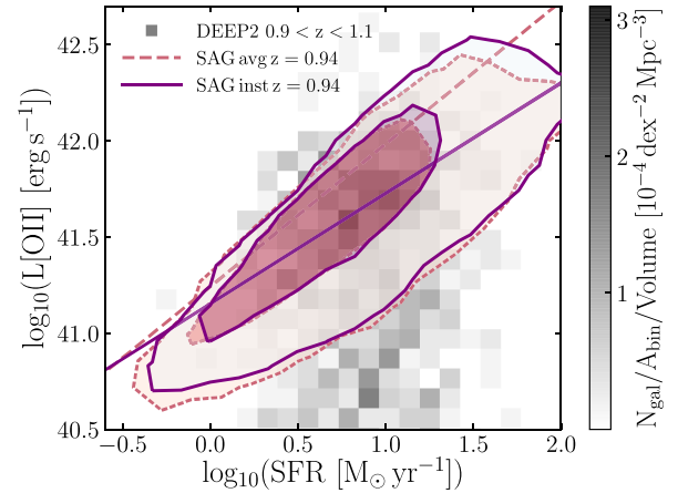
Figure A1. Non-attenuated [\text{O II}] luminosity as a function of SFR for the SAG model galaxies at z \sim 1 (contours) and the DEEP2-FF observations at 0.9 < z < 1.1 (grey, shaded squares). The colour bar represents the observed galaxy number density in each 2D bin normalised by the bin area in units of [\text{dex}^{-2} \text{ Mpc}^{-3}] . Here the SAG model galaxies are selected following the spline fit to the observed DEEP2-FF L[\text{O II}] distribution shown in Fig. 4. The model L[\text{O II}] values are calculated by assuming instantaneous (solid, purple contours) and average (dashed, salmon) SFR as input for the GET_EMLINES prescription. The innermost (outermost) model contours encompass 68 per cent (95 per cent) per cent of the galaxy distributions. The diagonal lines represent the L[\text{O II}] -SFR correlations, whose coefficients are reported in Table A1.
