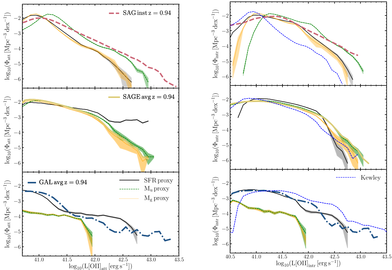
Figure 13. Left column: From top to bottom, attenuated [O II] LFs of the SAG, SAGE, and GALACTICUS model galaxies at z \sim 1 . We show as thick lines the results with L[\text{O II}] computed using the GET_EMLINES code described in Section 3.1 with either instantaneous or average SFR and metallicity as inputs. We compare these results with the L[\text{O II}] functions derived from the three L[\text{O II}] proxies established above: SFR (solid, black line), M_u (dashed, green), and M_g (dotted, orange). The shaded regions represent the \pm\sigma_y scatter in the proxy- L[\text{O II}] linear scaling laws, which is given in Table 2. Right column: Same as left column, but here the L[\text{O II}] are intrinsic. The lines are colour coded as the left-hand panels. We show as blue dashed lines the results from the Kewley et al. (2004) conversion.
