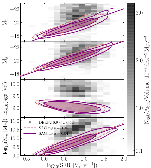
Figure A2. From top to bottom: intrinsic magnitudes, ages and stellar masses as a function of SFR for SAG model galaxies at z \sim 1 (contours) and DEEP2-FF observations at 0.9 < z < 1.1 (grey, shaded squares). The model galaxies have been selected following the observed DEEP2-FF distribution approximated by a spline fit, as explained in Section 2.2.2. The colour bar shows the number density of DEEP2 galaxies per bin area in units of [\text{dex}^{-2} \text{Mpc}^{-3}] . The dashed, salmon (solid, purple) contours represent the average (instantaneous) SFRs. The innermost (outermost) contours encompass 68 per cent (95 per cent) of the distributions. The diagonal lines are the linear fits showing the significant correlations, whose coefficients are reported in Table 2, together with the best-fitting parameters.
