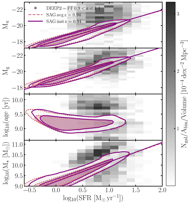
Figure 8. From top to bottom: intrinsic magnitudes, ages, and stellar masses as a function of SFR for SAG (contours) at z \sim 1 and DEEP2-FF observations at 0.9 < z < 1.1 (grey, shaded squares). The colour bar shows the number density of DEEP2 galaxies per bin area in units of [\text{dex}^{-2} \text{Mpc}^{-3}] . The dashed, salmon (solid, purple) contours represent the average (instantaneous) SFRs. The innermost (outermost) contours encompass 68 per cent (95 per cent) of the distributions. The diagonal lines are the linear fits showing the significant correlations (i.e. r \geq 0.6 ), whose coefficients are reported in Table 2, together with the best-fitting parameters.
