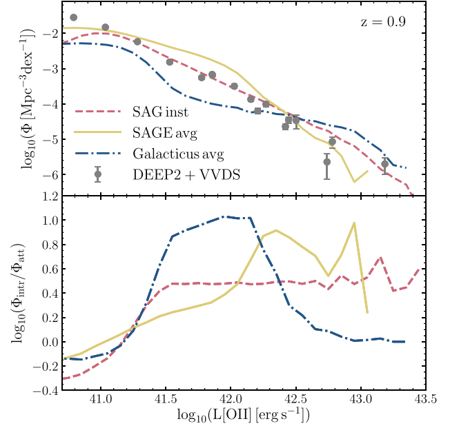
Figure 9. Top: Dust attenuated [O II] LFs of the MultiDark-Galaxies at z \sim 1 compared with DEEP2 + VVDS observations (Comparat et al. 2016). We consider all SAM galaxies above 5 \times 10^{-18} \text{ erg s}^{-1} \text{ cm}^{-2} . All the [O II] luminosities are computed using the GET_EMLINES code with SFR and cold gas metallicity as inputs (see Section 3.1). The SAG L[\text{O II}] , which are estimated using the instantaneous SFR, are in good agreement with the SAGE and Galacticus results based on the average SFR. Bottom: Ratios between the model intrinsic [O II] LFs (given by equation 8) and the dust attenuated ones (see Section 3.2) shown in the upper panel.
