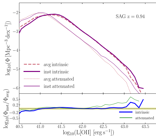
Figure 7. Intrinsic (thick lines) and attenuated (thin) [O II] LFs based on SAG average (dashed, salmon) and instantaneous SFR (solid, purple). The bottom panel shows the ratios between the two and the yellow stripe highlights the 5 per cent region of agreement. We apply the mocks the same [O II] flux limit of DEEP2-FF observations, 5 \times 10^{-18} \text{ erg s}^{-1} \text{ cm}^{-2} (see Section 2.2.2).
