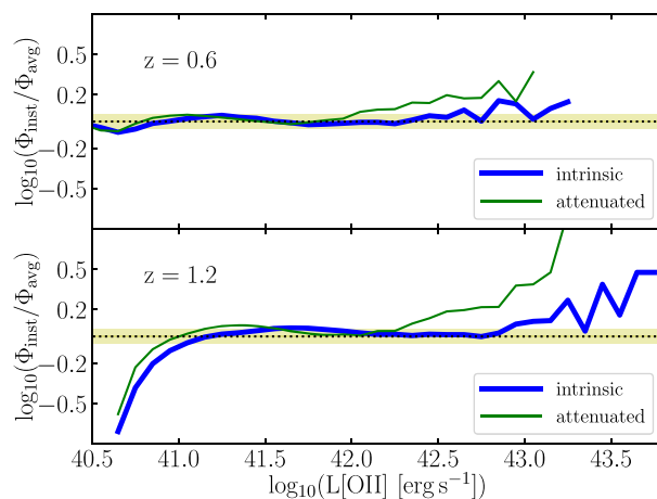
Figure B1. Ratios between the SAG [\text{O II}] LFs (thick, blue lines: intrinsic LFs; thin, green: attenuated LFs) at different redshifts computed from average and instantaneous SFR using the method presented in 3.1. The yellow, shaded areas represent the 5 per cent confidence region.
