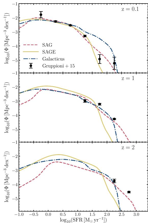
Figure 2. MultiDark-Galaxies average SFR function evolution at z \lesssim 2 (lines) compared to the Herschel/PEP and HerMES observations (Gruppioni et al. 2015, filled circles).
