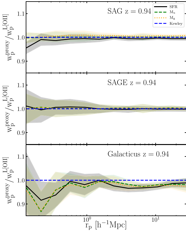
Figure 14. Proxy-to- L[\text{O II}] ratios of the projected two-point correlation functions of, from top to bottom, SAG, SAGE, and GALACTICUS model galaxies at z \sim 1 . The SAG L[\text{O II}] is estimated using the GET_EMLINES code with instantaneous SFR, while SAGE and GALACTICUS use the average quantity. Galaxies have been selected to have L[\text{O II}] > 10^{40.4} erg s ^{-1} . The shaded regions represent the effect of the \sigma_y scatter in the proxy- L[\text{O II}] linear relations reported in Table 2. These regions are the 1\sigma uncertainties derived from the covariance of 100 Gaussian realizations with the L[\text{O II}] proxy considered as mean and \sigma_y as scatter. We over plot the Kewley et al. (2004) result as a dashed, blue line.
