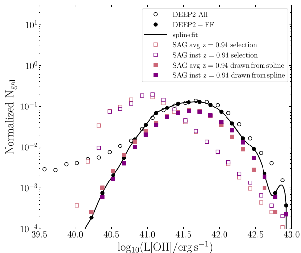
Figure 4. Attenuated L[\text{O II}] distribution of the original DEEP2 sample (black, empty dots) compared to the DEEP2-FF selection (black, filled dots), which we fit with a spline function. The area under the curves is normalized to unity. We compare these results with the SAG model galaxies selected with M_* > 10^{8.87} M_\odot and \text{SFR} > 0 \text{ yr}^{-1} M_\odot (empty squares; see Section 2.1.4), and with the SAG galaxies randomly drawn from the DEEP2-FF spline distribution (filled squares). The [O II] luminosity values in the model galaxies are calculated using the GET_EMLINES code, inputting either the instantaneous (purple) or average (salmon) SFR. All the details about these quantities and the calculations are given in Section 3.1.
