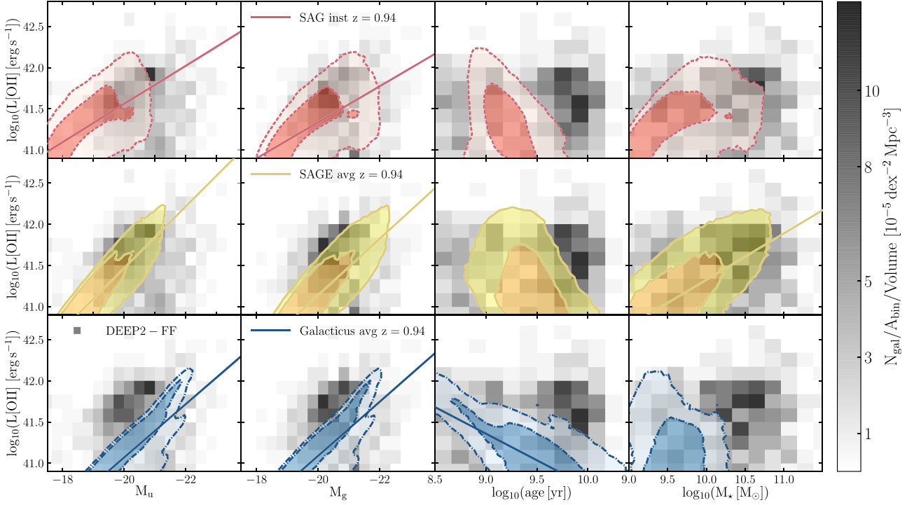
Figure 12. From top to bottom and from left to right: SAG, SAGE and GALACTICUS z \sim 1 intrinsic [O II] luminosities versus broad-band magnitudes, ages, and stellar masses (contours) compared with the DEEP2-FF observations at 0.9 < z < 1.1 (grey, shaded squares). The L[\text{O II}] values are computed using the GET_EMLINES code with instantaneous SFR for SAG and average SFR for SAGE and GALACTICUS. The innermost and outermost model contours represent 68 per cent ( 1\sigma ) and 95 per cent ( 2\sigma ) of the distribution. A minimum [O II] flux cut of 5 \times 10^{-18} \text{ erg s}^{-1} \text{ cm}^{-2} has been applied to both data and model galaxies. The diagonal lines are the linear fits for strong correlations with r > 0.6 , as reported in Table 2.
