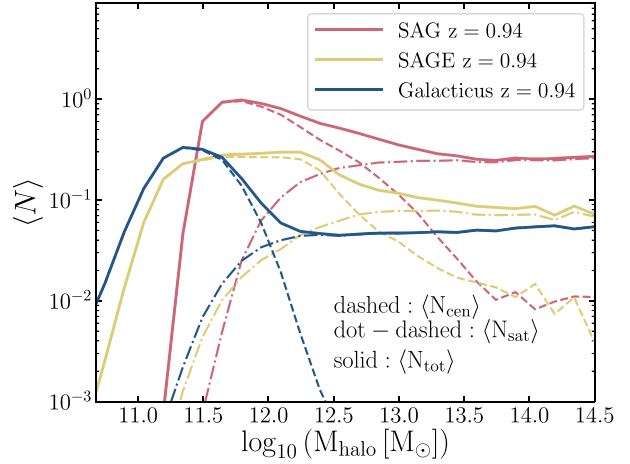
Figure 15. Mean HOD of the SAG (salmon solid line), SAGE (yellow solid line), and GALACTICUS (blue solid line) model galaxies with L[\text{O II}] > 10^{40.4} erg s ^{-1} at z \sim 1 . The model L[\text{O II}] has been computed using GET_EMLINES with instantaneous SFR for SAG galaxies and average SFR for SAGE and GALACTICUS. The contribution from central galaxies is shown by dashed lines and that for satellites by dot-dashed lines.
