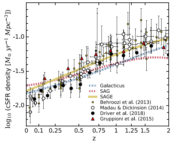
Figure 1. Cosmic SFR density of SAG, SAGE, and GALACTICUS MultiDark-Galaxies as a function of redshift, compared to four independent compilations of data sets from Behroozi, Wechsler & Conroy (2013) [this was corrected to a Chabrier, Hennebelle & Charlot (2014) IMF by the same authors], Madau & Dickinson (2014), Driver et al. (2018), and Gruppioni et al. (2015). The error bars are the 1\sigma dispersion around each point. We show this result only up to z \sim 2 , which is the maximum redshift of interest for our study.
