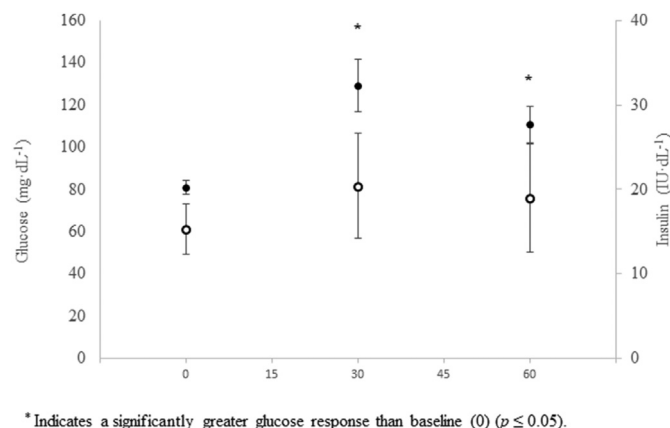
Fig. 2. Means \pm 95% Confidence Intervals of glucose (closed circles) and insulin (open circles) responses of pre-pubescent children (n = 19) measured at baseline and 30 and 60 min after consuming a 30-g RDC drink.
