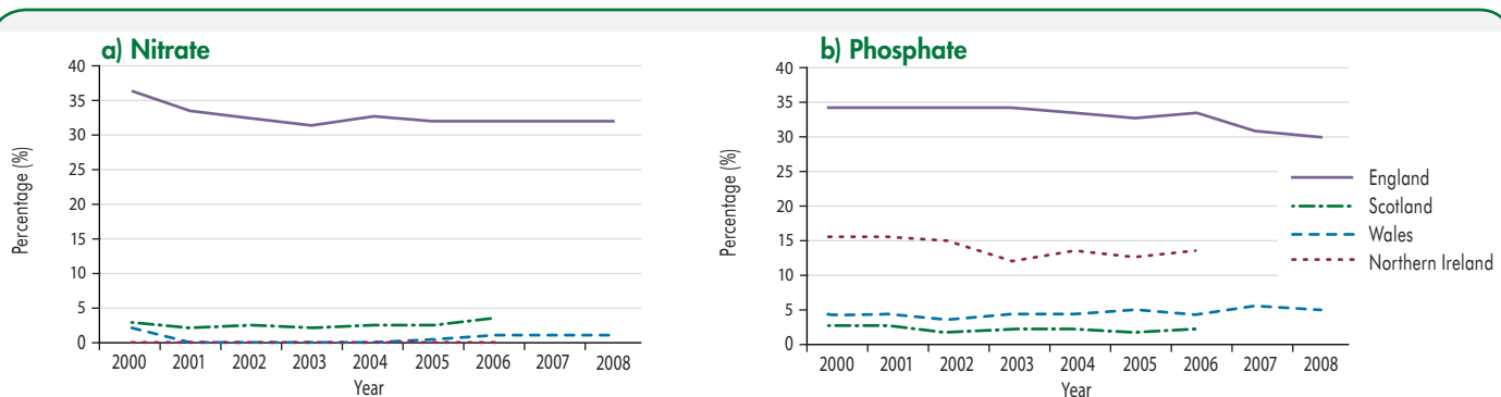
Figure 7.11 Percentage of river lengths in England, Scotland, Wales and Northern Ireland with high levels of a) nitrate ( \text{NO}_3^* ; levels greater than 30 mg \text{NO}_3/\text{l} ) and b) phosphate (P; levels greater than 0.1mg P/l) from 2000 to 2008. * Note: no values for Northern Ireland exceeded zero. Source: Defra (2010a) © Crown copyright.
