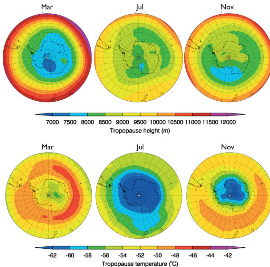
Figure 9. Monthly climatologies of (top) blended tropopause height (m) and (bottom) temperature (°C) from the ERA-Interim climatology (1989–2007) for SH high latitudes (40–90°S) in March, July and November.
