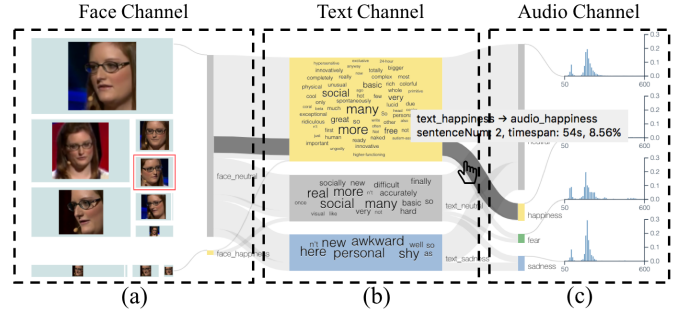
Fig. 5: An augmented Sankey diagram design for summarizing emotion coherence from three channels as well as for providing extracted features for explanations. Each node represents one type of emotion and each link represents a collection of sentences with certain emotions shared by two channels, either the face and text channels or the text and audio channels. (a) A treemap-based design to show a quick overview of representative detected faces in the video. (b) A word cloud design to highlight some important words, which gives users some hints about the corresponding context. (c) A histogram design to show the audio feature distribution for different emotions.
