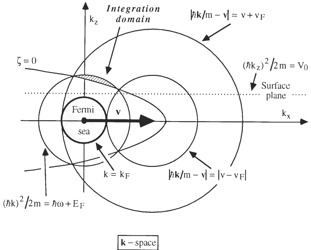
Figure 10. Region of non-vanishing values of \xi in eq. (20). \xi = 1 inside the dashed region. The plane of representation of the figure is perpendicular to the k_y axis. All curves have cylindrical symmetry with respect to the k_x axis, except the surface plane, which is perpendicular to the k_z axis.
