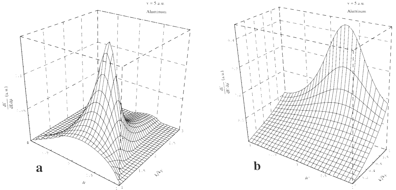
Figure 2. (a) Doubly differential electron excitation rate due to the interaction of a homogeneous electron gas with a unit charge moving with constant velocity v = 5 a.u., according to eq. (7). The momentum and direction of motion of the electron are given by \hbar\mathbf{k} and \mu = \cos(\mathbf{k}, \mathbf{v}) , respectively. The Mermin dielectric function [40] has been used to represent the response of the medium. Electron gas parameters appropriate to aluminum have been utilized (one-electron radius r_s = 2.07 a_0 and damping \hbar\gamma = 1.35 eV). (b) Under the same conditions, creation rate of holes of momentum \hbar\mathbf{k}' around the direction \mu' = \cos(\mathbf{k}', \mathbf{v}) , according to eq. (8).
