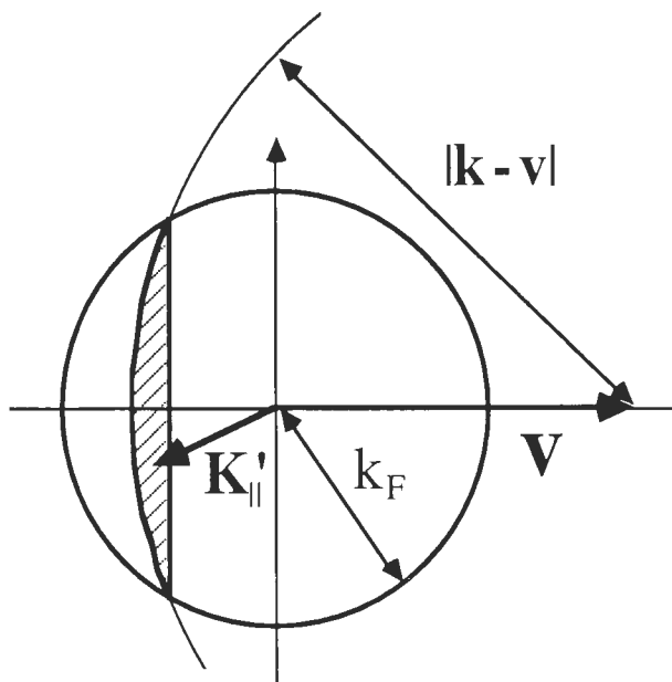
Figure 7. Domain of integration in eq. (18) in the K'_{\parallel} -plane. \hbar\mathbf{k} is the electron momentum inside the solid.
