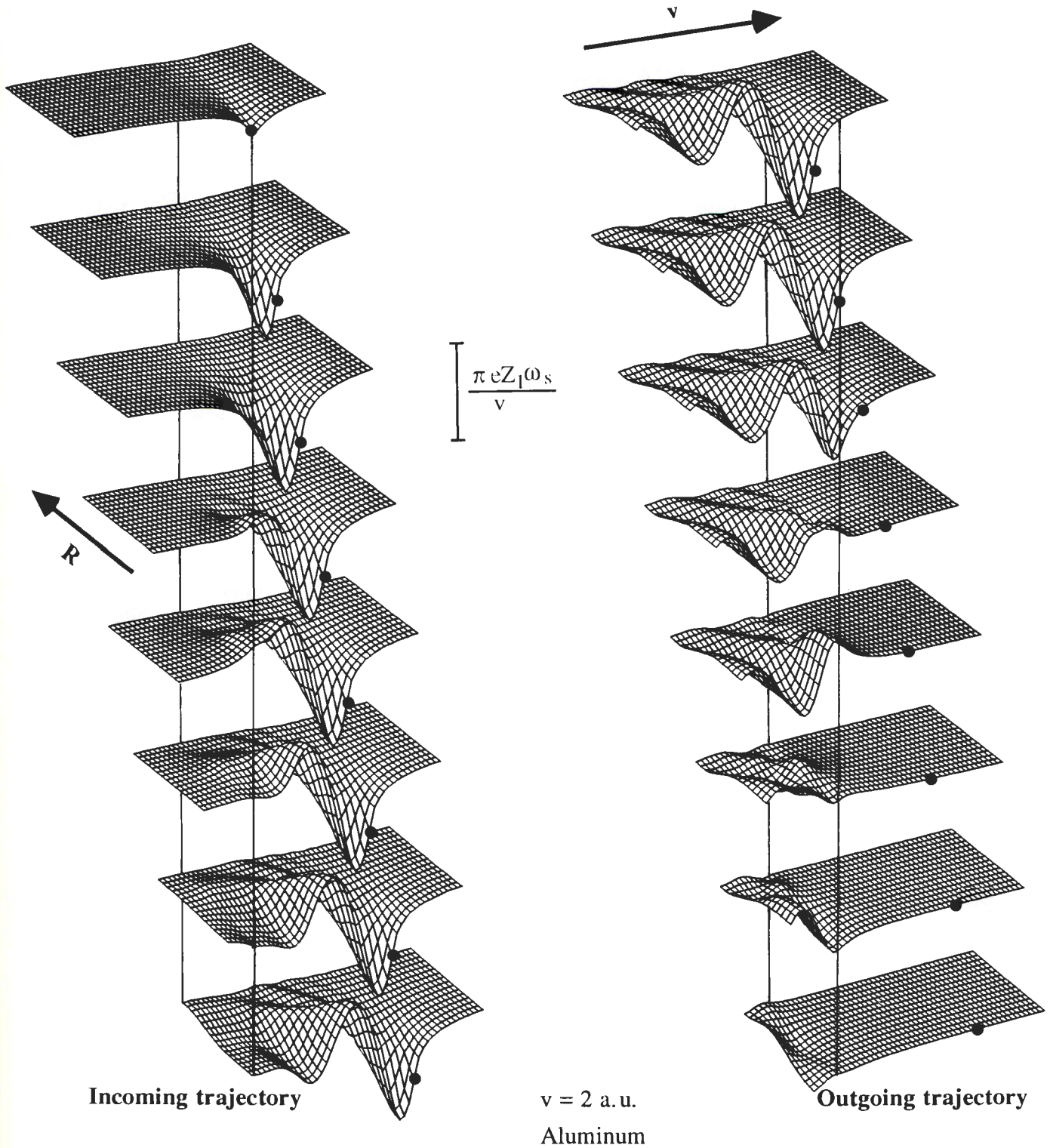
Figure 4. Induced surface wake potential created by a charged particle of charge eZ_1 moving with constant velocity v = 2 \text{ a.u.} perpendicular to an aluminum surface for the cases of incoming (left) and outgoing (right) trajectories. The surface is represented by vertical lines, with the medium located on the right/left side in the incoming/outgoing trajectory. The dimensions of each grid are 50 \times 15 \text{ a.u.} (i.e., 26.4 \times 7.9 \text{ \AA} ). The subdivisions in the grids correspond to squares of side 1 \text{ a.u.} The particle (black circles) is moving from left to right. R is the direction perpendicular to the trajectory.
