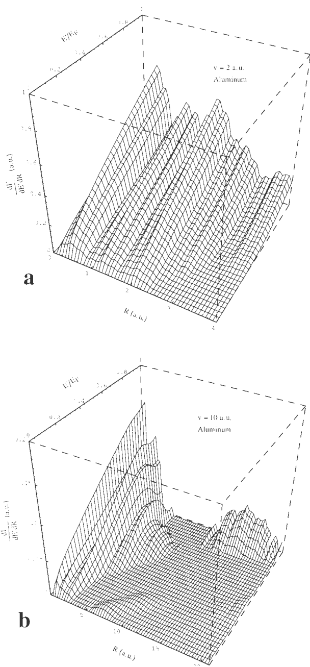
Figure 16. Spatial representation of the rate of creation of holes shown in Figure 2b, calculated by integration of eq. (30) over E , for v = 2 a.u. and v = 10 a.u.
