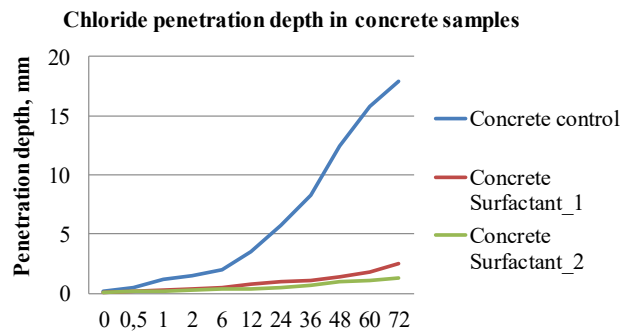
Fig. 3. The penetration depth of chlorides into concrete samples, with an exposure of 0–72 hours
