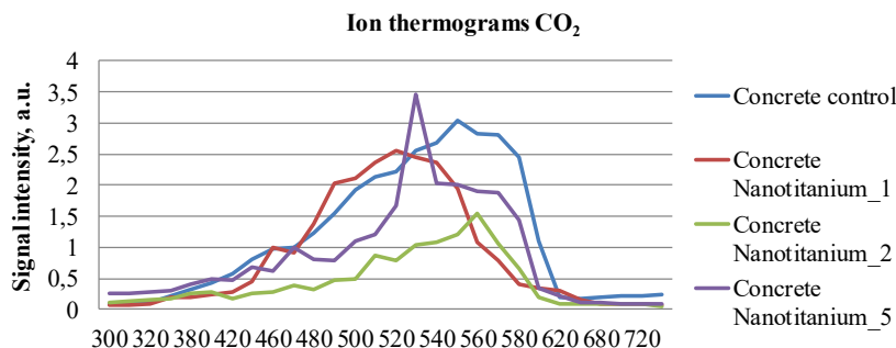
Fig. 5. Thermograms of CO 2 emission/elimination ( m/z=44 ) by thermal decomposition of a sample
