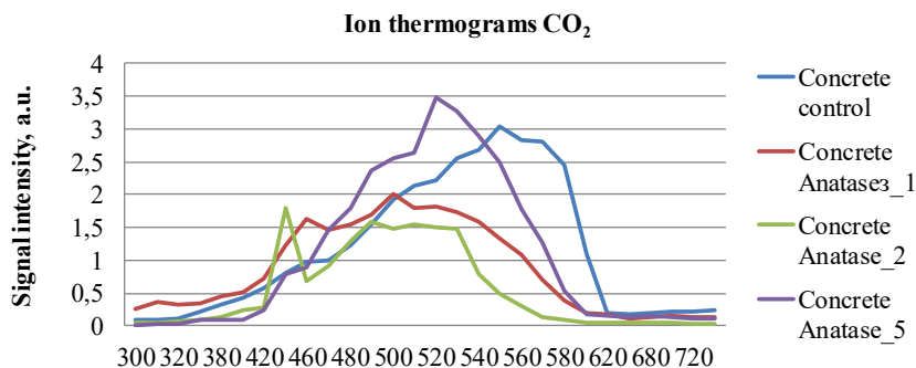
Fig. 6. Thermograms of CO 2 emission/elimination ( m/z=44 ) by thermal decomposition of a sample
