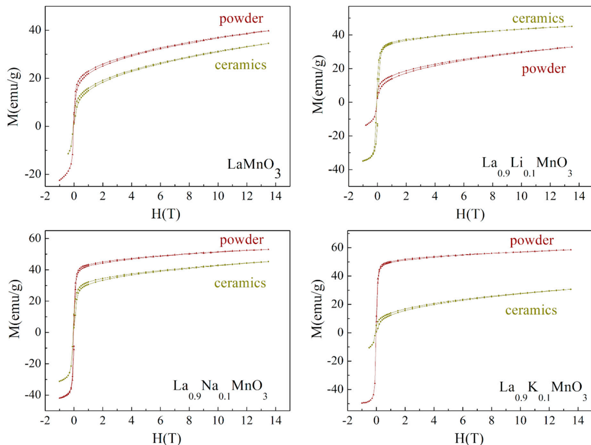
Figure 6. Isothermal magnetization curves measured for the initial compound \text{LaMnO}_3 and doped \text{La}_{0.9}\text{A}_{0.1}\text{MnO}_3 (A: Li—right top, Na—left bottom, K—right bottom) powder and ceramics at T = 5 K.
