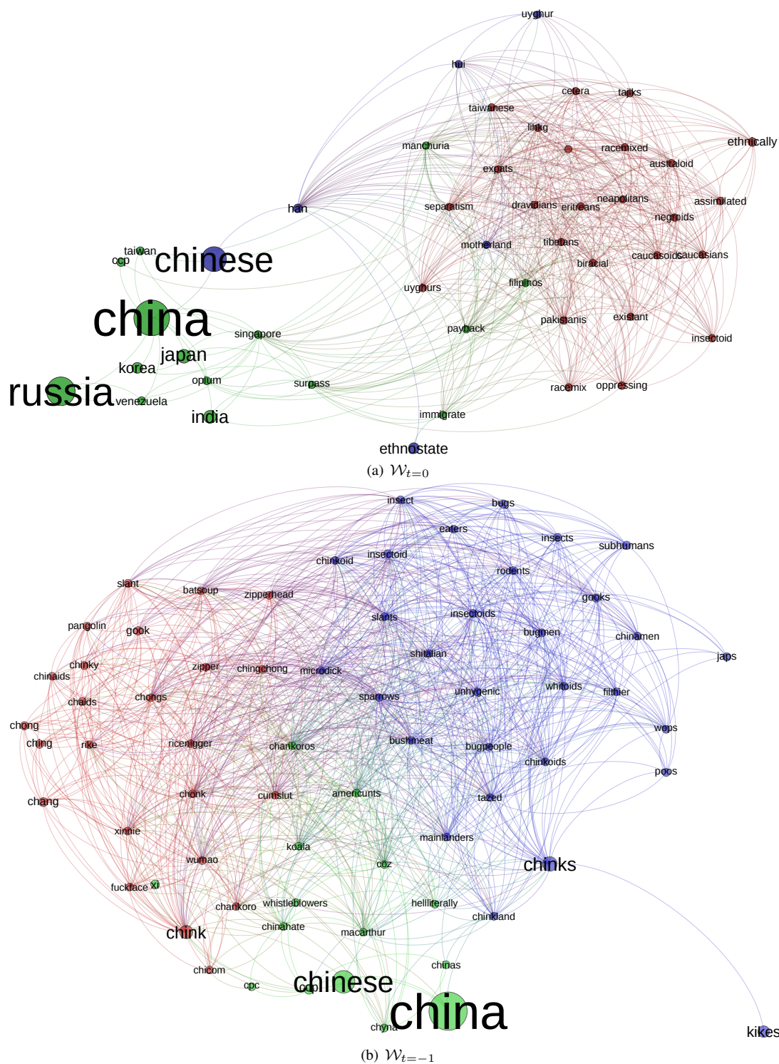
Figure 8: Visualization of a 2-hop graph from the word “chinese” on 4chan’s /pol/ using the first and last weekly word2vec models.
