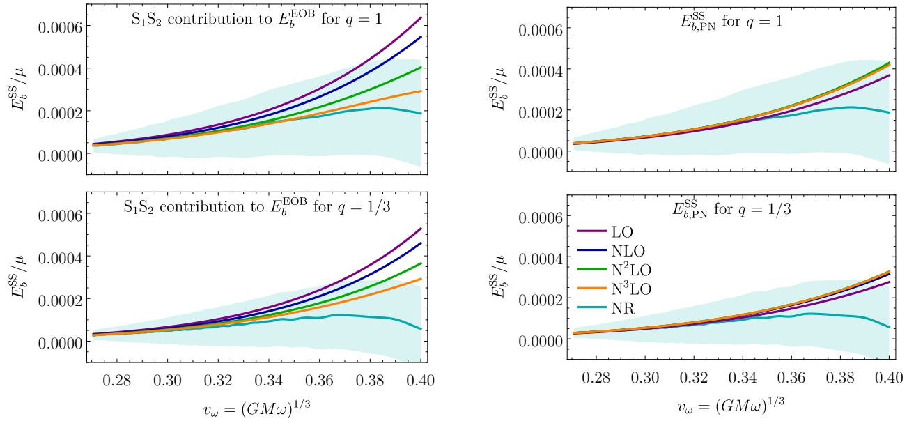
FIG. 2. Binding energy versus the velocity parameter v_\omega for the S_1S_2 contribution to the EOB (left panels) and PN-expanded (right panels) binding energies for mass ratios q = 1 (top panels) and q = 1/3 (bottom panels). The NR error is indicated by the shaded regions.
