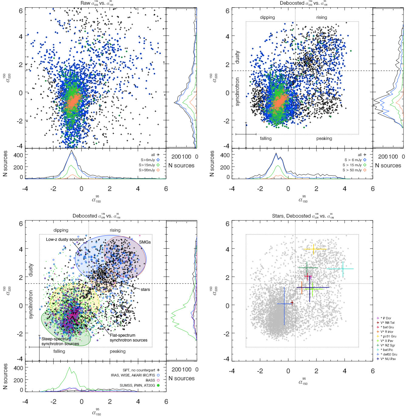
Figure 4. Upper panels: raw (left) and deboosted (right) \alpha_{150-220} vs. \alpha_{95-150} , where colors and symbols indicate flux level. Dotted box indicates the bounds of the prior on spectral index applied during deboosting, and dotted horizontal and vertical dashed lines indicate \alpha_{150-220} = 1.51 , the minimum of the 150-220 GHz summed posterior and the corresponding separation index between dusty and synchrotron in 95-150 GHz from reexamining the distributions of summed spectral index posteriors after population separation. These separation lines are used to categorize sources into four quadrants of “falling,” “rising,” “peaking,” and “dipping.” The typical error for a source at the 4.5- \sigma detection threshold is shown in the lower left corner of the deboosted spectral index plots. Lower panels: Left: deboosted \alpha_{150-220} vs. \alpha_{95-150} , where colors and symbols indicate cross-matches with external catalogs, and black crosses indicate SPT sources with no cross-matches in external catalogs. Right: Measured spectral indices for ten stars detected in the catalog, overplotted on the rest of the catalog, shown by grey crosses.
