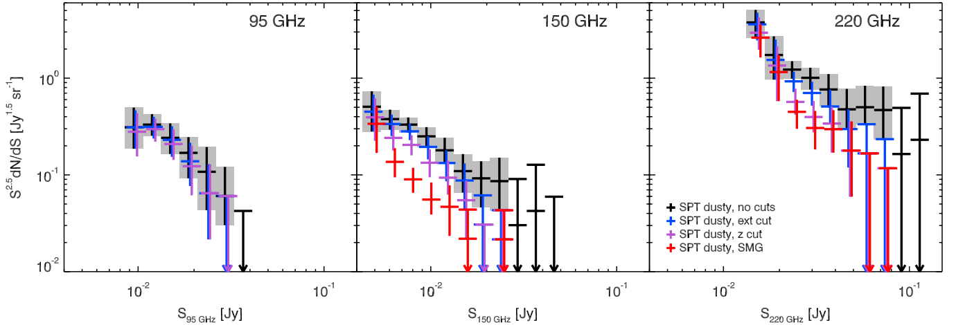
Figure 20. Number counts of SPT dust-dominated sources, showing a comparison of different cut versions. All sources identified as stars have been removed from the catalog prior to the counts calculation. Four cut versions are shown: 1) only stars have been removed, “no cuts.” 2) Cutting all stars and all sources flagged as extended or detected as multiple detections and confirmed to be from a single object, “ext cut,” 3) cutting all sources with measured redshifts z < 0.1 , “ z cut,” and 4) the SPT SMG list, cutting all sources with measured redshifts, IRAS cross-matches, or dipping spectral behavior in the SPT bands.
