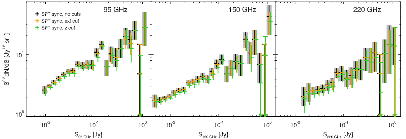
Figure 19. Number counts of SPT synchrotron-dominated sources, showing a comparison of different cut versions. All sources in the catalog that are identified as stars have been removed from the catalog prior to the counts calculation. Three cut versions are shown: 1) only stars have been removed, “no cuts.” 2) Cutting all stars and all sources flagged as extended or detected as multiple detections and confirmed to be from a single object, “ext cut,” and 3) cutting all sources with measured redshifts z < 0.1 , “z cut.”
