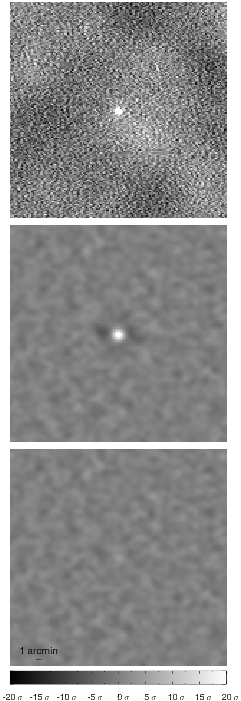
Figure 2. A demonstration of the CLEAN method showing a single example source detected at 22.4\sigma in RA4H10DEC-50 at 150 GHz, showing cutouts from the raw, coadded map ( top ), optimally-filtered map ( middle ), and residual map ( bottom ), scaled for illustration by the mean RMS map noise for the sector containing this source. We note that since we CLEAN down to a threshold of 4.5\sigma , there is flux remaining in the residual map at the source location, at a significance of roughly 4.4\sigma , just below the detection threshold.
