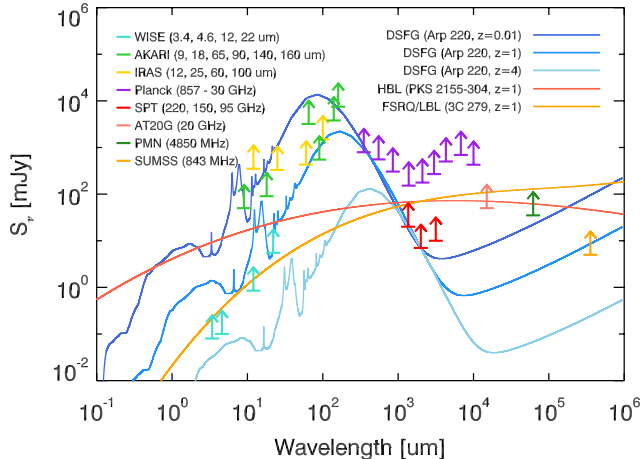
Figure 7. A comparison of survey depths for SPT and wide-field surveys used to cross-match with the SPT source catalog. Blue curves show example spectral energy distribution (SED) curves for dusty star-forming galaxies and their high-redshift component, SMGs, which are an Arp 220 SED shifted in redshift. Red and orange curves show two example synchrotron SEDs for different types of flat-spectrum sources.
