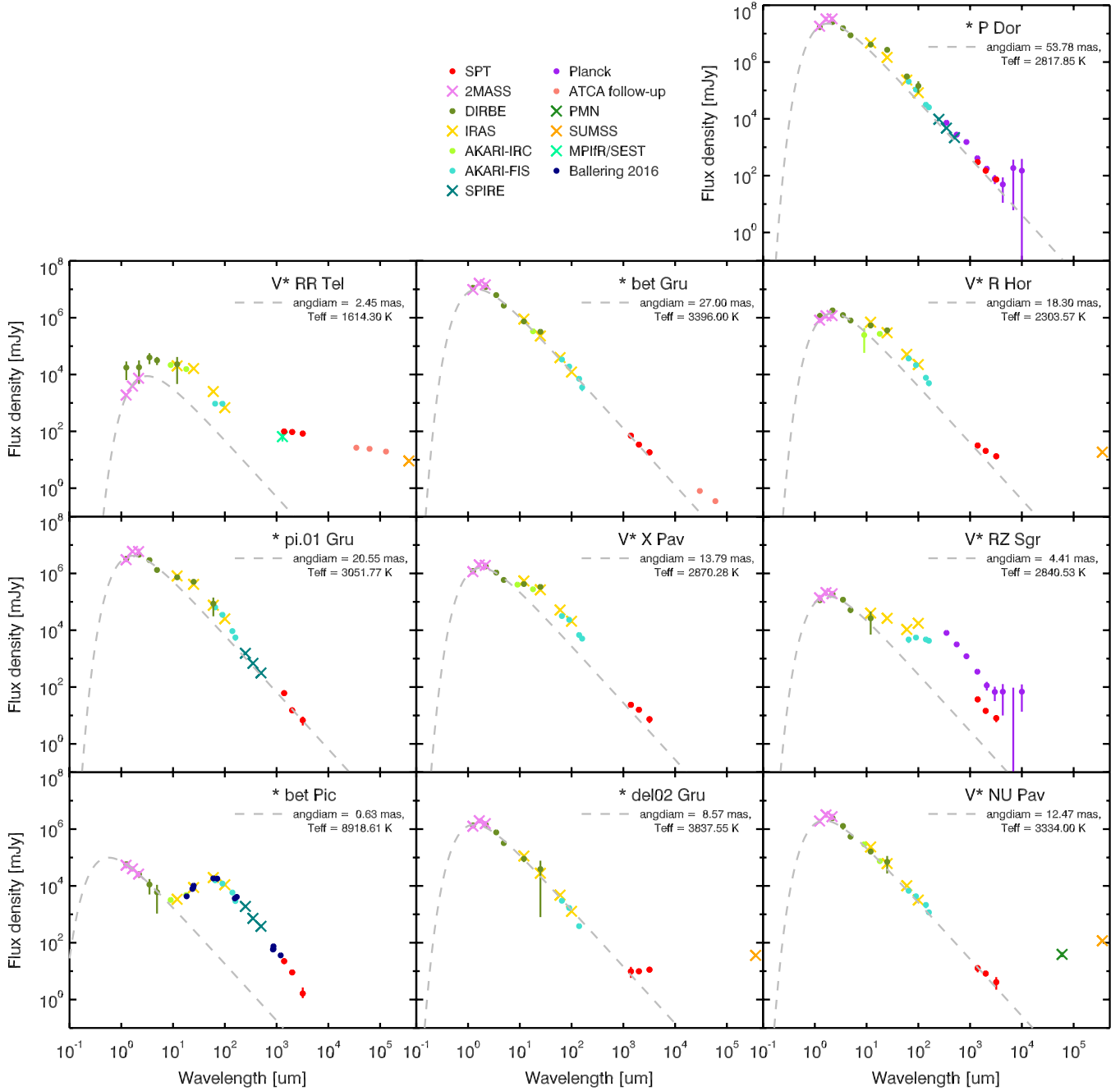
Figure 13. Spectral energy distributions for the ten stars detected in the SPT-SZ catalog, with flux measurements drawn from the literature. Grey dashed lines show blackbody model fits, where only fluxes from wavelengths in the range 1.25 - 5 \mu\text{m} are used in the fit. In addition to available statistical errors from the literature, 10% absolute calibration uncertainties have been applied to all fluxes from the literature.
