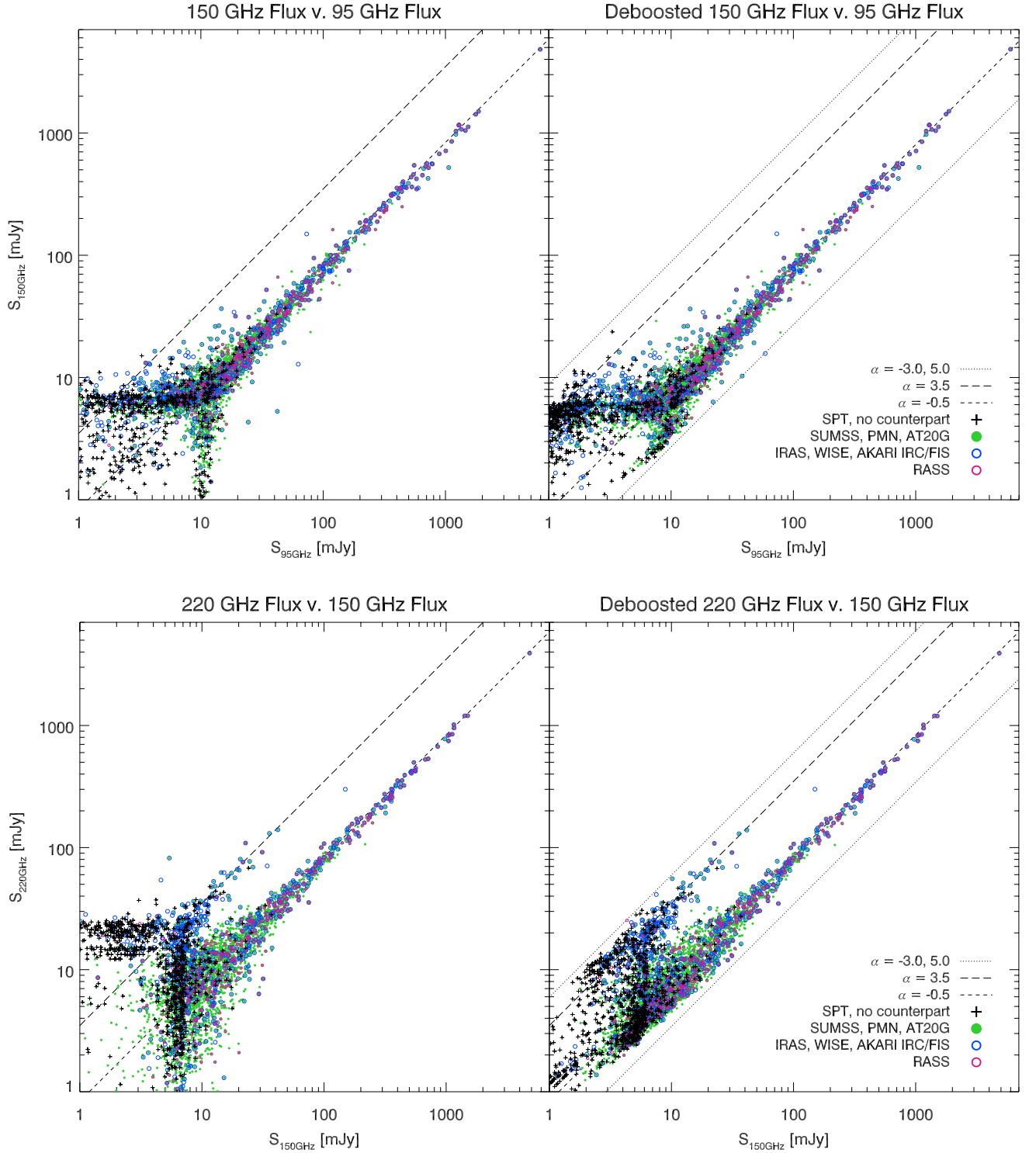
Figure 3. Upper panels: raw ( left ) and deboosted ( right ) fluxes for 150 GHz vs. 95 GHz for all sources in the catalog. Lower panels: raw ( left ) and deboosted ( right ) fluxes for 220 GHz vs. 150 GHz. Colors and symbols show cross-matches with external catalogs and black crosses indicate sources detected by the SPT-SZ survey with no counterparts in external catalogs. Dashed lines show expected spectral indices for synchrotron and dusty populations, and dotted lines in the right panels show bounds applied as priors on spectral index for the deboosting. The vertical and horizontal clusters of sources at relatively low flux in the left panels show the detection thresholds of 4.5\sigma , which translate to a different flux threshold for each field. For example, the clusters at clearly different flux levels in 220 GHz represent the 4.5\sigma thresholds in the double-depth fields and in the rest of the catalog.
