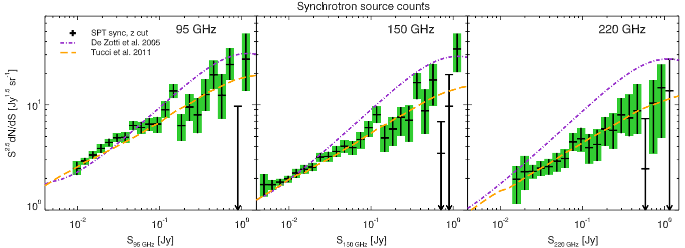
Figure 14. Differential number counts of SPT synchrotron-dominated sources. All sources in the catalog that are identified as stars as well as all sources flagged with the “z cut” (i.e. sources with measured redshifts z < 0.1 ) have been removed from the catalog prior to the counts calculation. A comparison of the effects of different cut versions on the number counts can be found in the appendix. Overplotted are the De Zotti et al. (2005) and the Tucci et al. (2011) models, which have not been fit to the SPT data.
