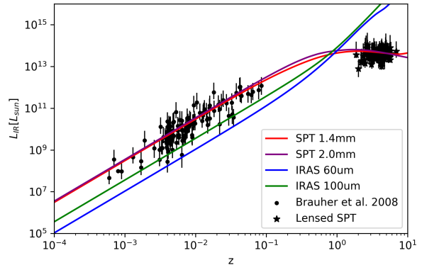
Figure 11. Observed infrared luminosity versus redshift for low-redshift infrared galaxies (Brauher et al. 2008) and SPT SMGs with detection thresholds for an Arp-220-like dusty galaxy spectrum shown in solid lines.
