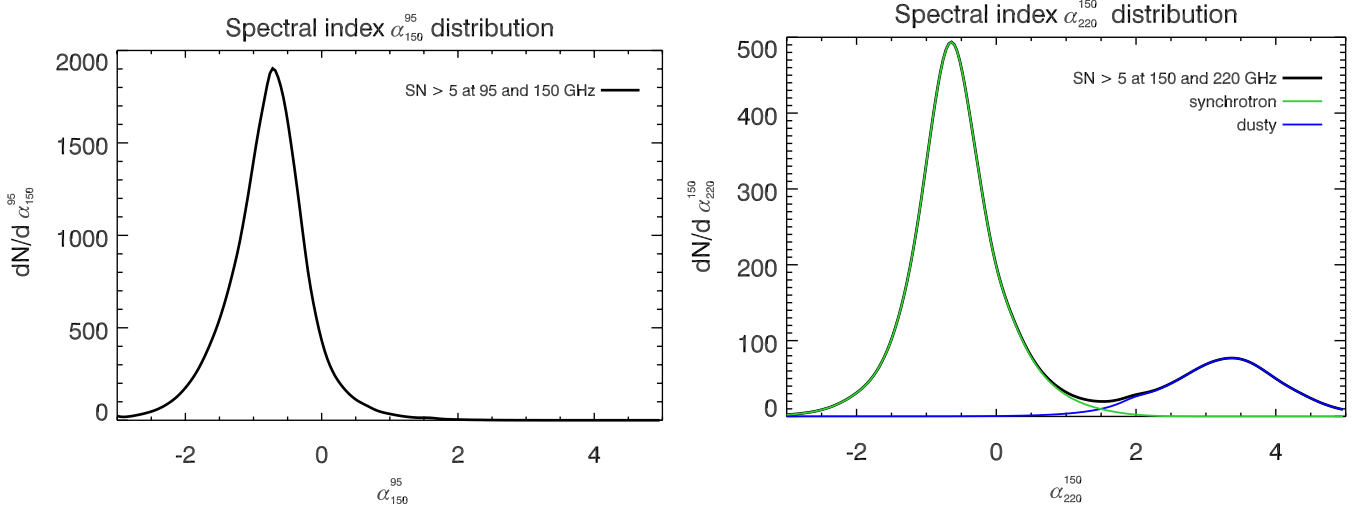
Figure 6. Summed normalized posterior distributions for the 95-150 GHz spectral index ( left ) and the 150-220 GHz spectral index ( right ), choosing for each spectral index only sources with detections above 5\sigma in both bands spanned by that index. As expected, the distribution for \alpha_{95-150}^{\max} shows a single peak at \alpha_{95-150}^{\max} \sim -0.7 \pm 0.6 , since synchrotron sources are expected to dominate at 95 GHz, especially for bright, and therefore high-signal-to-noise, sources. The distribution for \alpha_{150-220}^{\max} shows distinct peaks for synchrotron and dusty populations, with peaks at \alpha_{150-220}^{\max} \sim -0.6 \pm 0.6 and \alpha_{150-220}^{\max} \sim 3.4 \pm 0.8 , respectively, and we select the minimum at \alpha_{150-220}^{\max} = 1.51 as the threshold for applying a categorization for each source in the catalog.
