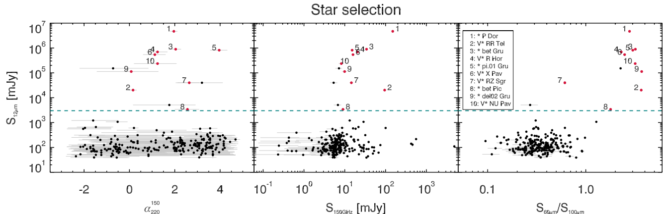
Figure 10. Cross-matched IRAS 12\ \mu\text{m} flux versus SPT spectral index \alpha_{150-220} ( left ), SPT flux at 150 GHz ( middle ), and the ratio of cross-matched IRAS 60\ \mu\text{m} flux to 100\ \mu\text{m} flux ( right ). Objects in the SPT-SZ catalog identified as stars are shown as red points, all other objects in the SPT-SZ catalog are shown as black points, with a rough separation threshold in 12\ \mu\text{m} flux shown as a teal dashed line. We note that using SPT data alone, stars are not distinguishable from non-stellar SPT sources (left two panels), and that while the ratio of 60\ \mu\text{m} to 100\ \mu\text{m} IRAS flux can be used to identify stars (right panel), high flux at 12\ \mu\text{m} is sufficient for star identification. The method for identifying stars is discussed in more detail in Section 4.9, and further details regarding stars identified in the SPT-SZ catalog and other sources that appear with high flux at 12\ \mu\text{m} but are not identified as stars can be found in Section 6.1.4.
