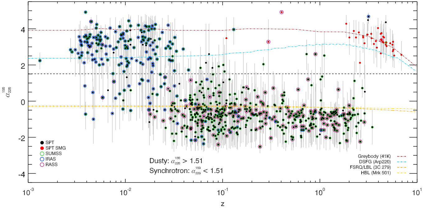
Figure 9. Deboosted \alpha_{150-220} versus redshift for sources in the SPT-SZ catalog with measured redshifts either from cross-matches in NED or follow-up observations with ALMA (Weiß et al. 2013; Strandet et al. 2016). Sources in the SMG list with measured redshifts are shown as red points, all other SPT-SZ catalog sources are shown as black points. The black dashed line shows the separation between dusty and synchrotron sources. Dot-dashed lines show two models of dusty sources: a 41 K greybody (red) and an Arp 220 model (blue), and two models of flat-spectrum synchrotron sources: a model for flat-spectrum sources dominated by radio emission (FSRQs and LBLs) based on the spectrum of the blazar 3C 279, and a model for flat-spectrum sources dominated by X-ray emission (HBLs) based on the spectrum of the blazar Markarian 501. Because redshifts are drawn from multiple sources, the selection function for SPT-SZ sources with measured redshifts is complicated. We don’t attempt to quantify the redshift completeness of the catalog, and this figure therefore is meant to illustrate the known redshift information for the catalog.
