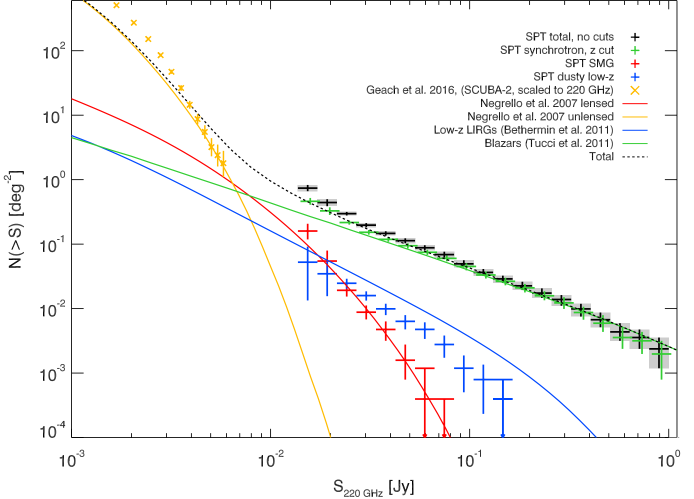
Figure 18. Cumulative number counts at 220 GHz for total, synchrotron-dominated, and dust-dominated source populations in the SPT-SZ catalog.
