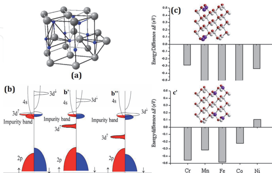
Figure 2. (a) Hexagonal wurtzite ZnO unit cell. Density of states (schematic) of \text{Zn}_{1-x}\text{TM}_x\text{O} , \text{TM} = \text{Ti} (b), \text{Mn} (b'), \text{Co} (b''), for which the Fermi level lies in a spin-split donor impurity band. (c) Energy differences, \Delta E = E_{\text{AFM}} - E_{\text{FM}} , for \text{Zn}_{0.857}\text{TM}_{0.143}\text{O} ( \text{TM} = \text{Cr}, \text{Mn}, \text{Fe}, \text{Co}, \text{and Ni} ) supercell; Zn (light gray spheres), O (red), and TM (purple) (adopted from [17–19]).
