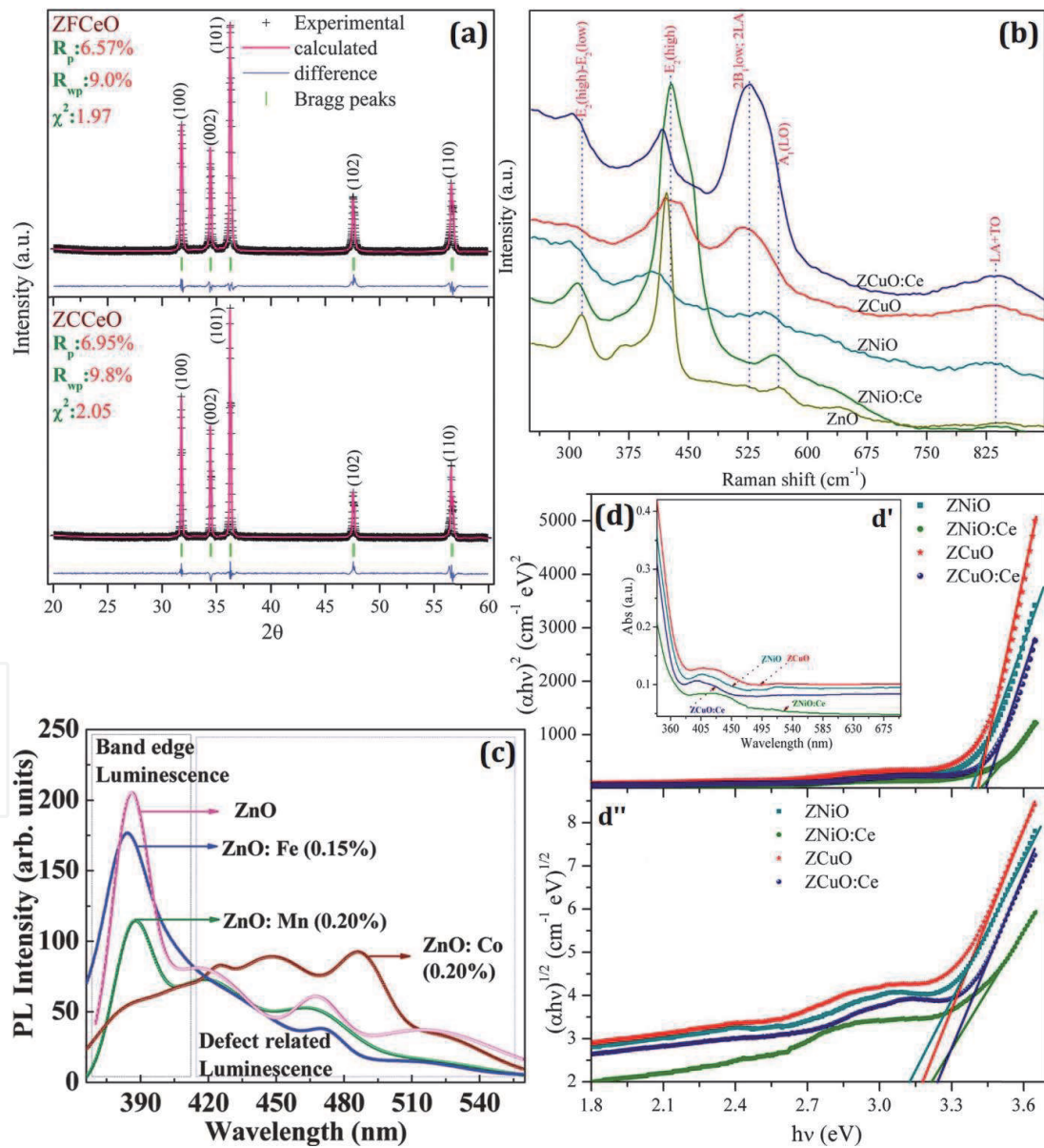
Figure 3. (a) XRD pattern of Zn_{0.94}Fe_{0.03}Ce_{0.03}O (ZFCeO) and Zn_{0.94}Co_{0.03}Ce_{0.03}O (ZCCeO) nanoparticles. (b, d) Raman and UV-visible absorption (for energy band calculation) spectra of Zn_{0.95}Ni_{0.05}O (ZNiO), Zn_{0.91}Ni_{0.05}Ce_{0.04}O (ZNiO/Ce), Zn_{0.95}Cu_{0.05}O (ZCuO), and Zn_{0.91}Cu_{0.05}Ce_{0.04}O (ZCuO/Ce) nanoparticles. (c) Photoluminescence spectra for ZnO with Co, Mn, and Fe nanoparticles (adapted from [27, 40, 41]).
