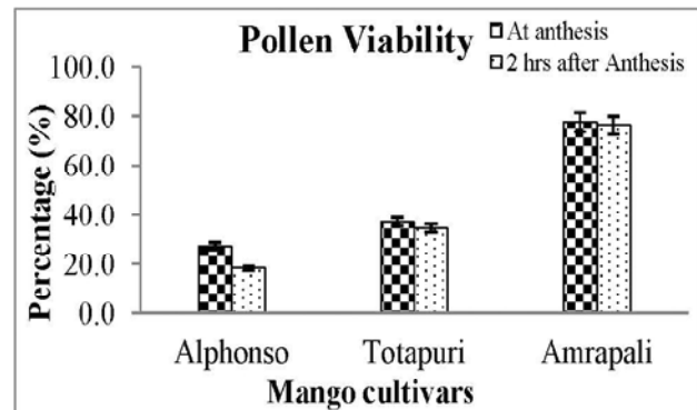
Fig 1. Pollen viability (% viable pollens) in cvs. Alphonso, Totapuri and Amrapali at anthesis and 2 hrs after anthesis
