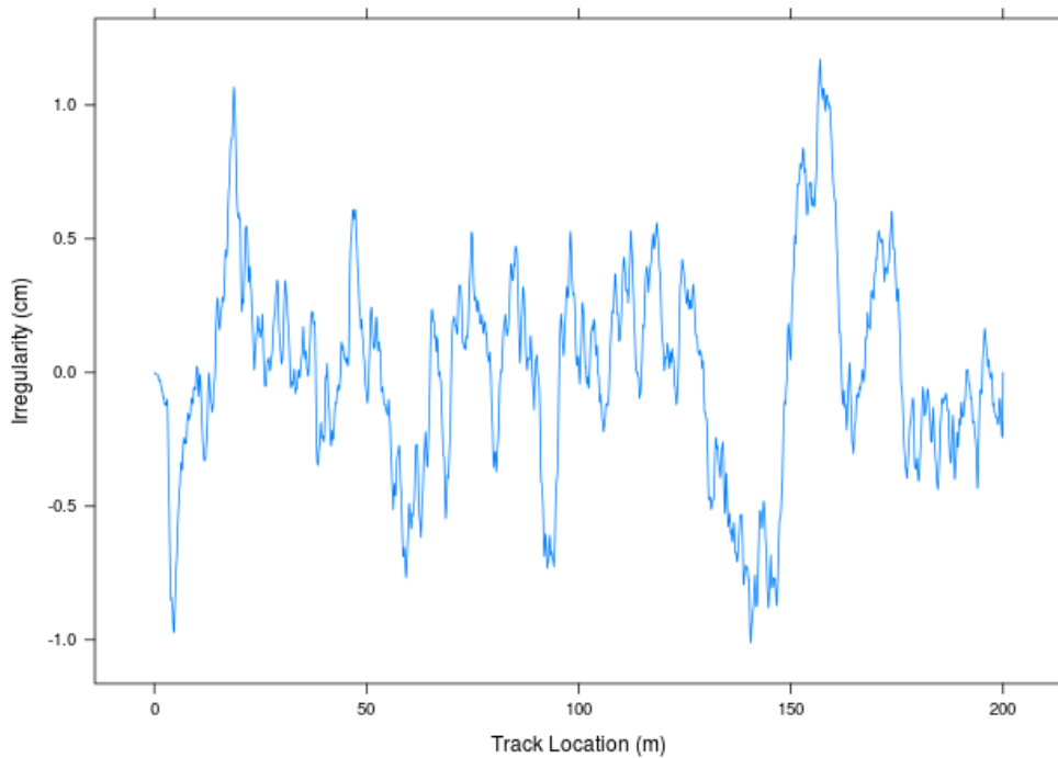
Figure 3. Vertical track irregularity profile
