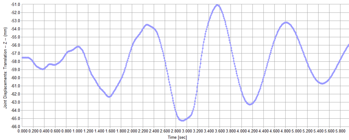
Figure 4. Vertical displacement at the center of the front car as a function of time. Although the cars have left the track at 4.51 sec, the vehicle remains a part of the analysis until the final time step with wheels assumed to have zero displacement.
