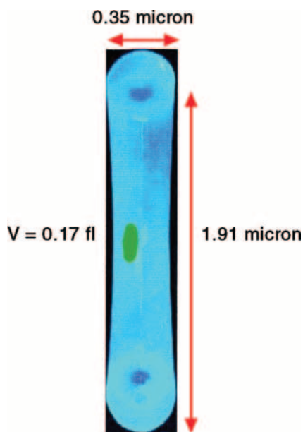
Fig. 1 Fluorescence correlation spectroscopy and two-color fluorescence cross-correlation spectroscopy detect the random Brownian motion of fluorescent molecules in a probe region of about 0.2 fl ( 0.2 \times 10^{-15} L) and less within the sample. The green fluorescent molecules, e.g. rhodamine green, diffuse in and out of the focal plane and thereby cause fluctuations in the fluorescence intensity. The process occurs, for example, with the natural frequency of k = \frac{P(X \leq 1; C = \Pi \cdot T) = P_1 = N}{\tau_{diff}} = \frac{0.0085}{26 \cdot 10^{-6}[\text{sec}]} = 326.92[\text{sec}^{-1}] . All parameters on the right hand side are measured by the (normalized) fluorescence intensity correlation curve. [4] k is the time constant of the mean value and the variance of the re-entry probabilities p_n(t) . [13] Thus, the self-same molecule re-enters the probe region 326.92 times per second. The portion of no meaningful re-entries that do not result in a useful burst size is 1 - 0.0085 = 0.9915 , i.e., 99.15%. [13] With the derived fraction of meaningful reentries, we obtain the meaningful time T_m Eq. (11), which is 3.06 ms under the experimental conditions. [13] For the individual complexed. Molecule of an antibody target in serum, the meaningful time T_m is 19.36 ms under the experimental conditions given in the main text. [13] (View this art in color at www.dekker.com .)
