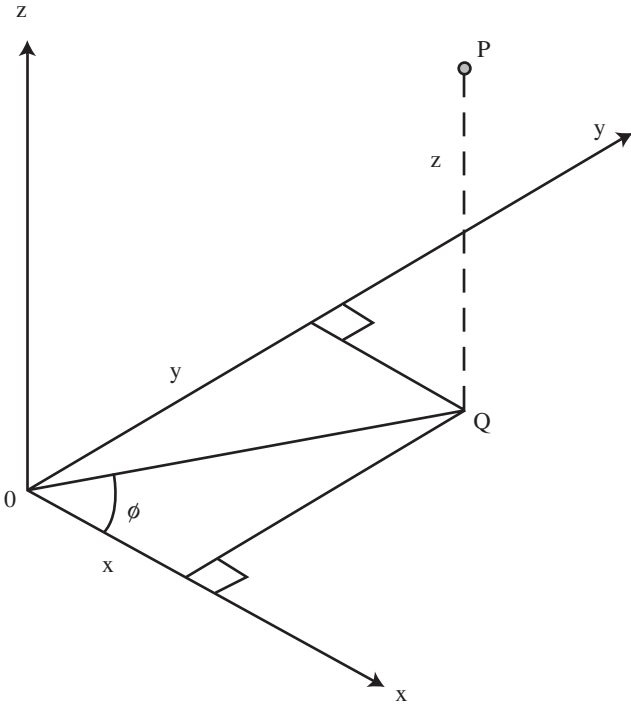
Fig. 2 The single molecule P in three dimensions has cylindrically polar coordinates (q, \phi, z) . Q is the foot of the perpendicular from the single molecule P into the focal x - y plane of the detection/observation volume. \phi is the angle between OQ and the x -axis. q is the length of OQ .
