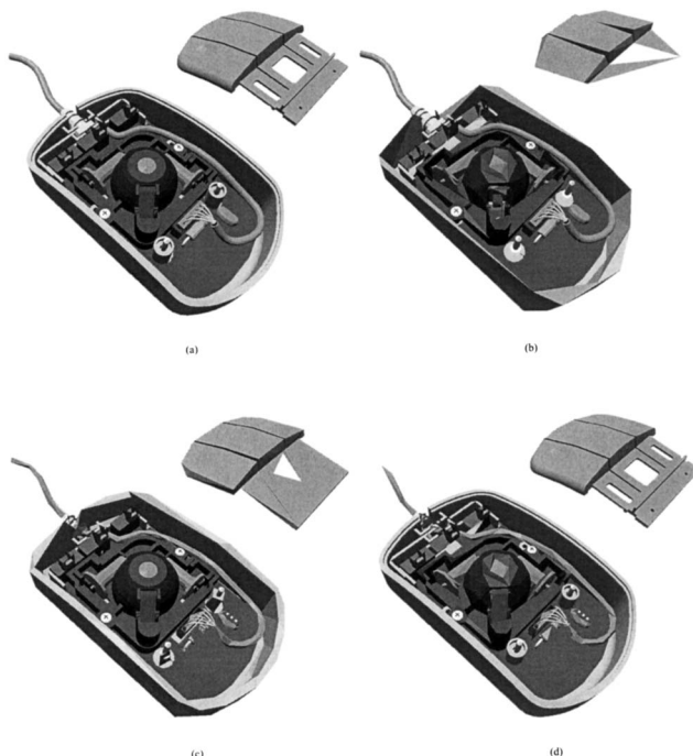
Fig. 9 Role-based views for the mouse assembly example. (a) The supervisor's ( a_0 ) full resolution view. (b) The electrical engineer's ( a_1 ) role-based view. The electrical features are displayed in full resolution, the mechanical features in a lower resolution, and the exterior features in an even lower resolution. (c) The mechanical engineer's ( a_3 ) role-based view. Mechanical features are displayed in full resolution, the electrical features in a lower resolution, and the exterior features in even lower detail. (d) The ergonomic engineer's ( a_5 ) role-based view. This depicts the interior and exterior in full resolution, but the remaining features are displayed in a low resolution.
