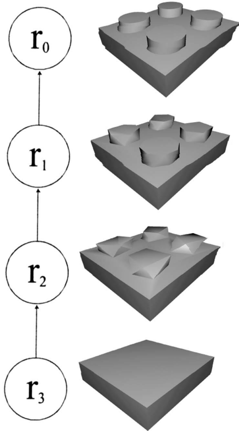
Fig. 5 An example part with one security feature ( f_0 ) consisting of b(M) assigned to r_0 , a set of actors assigned to roles, and their corresponding set of secure models
