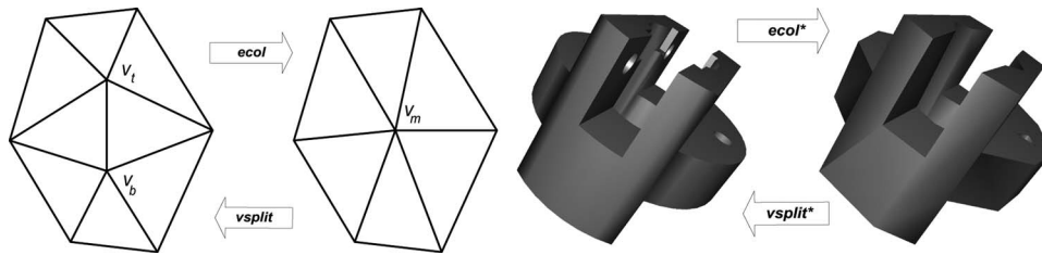
Fig. 1 Illustration of multiresolution techniques. (a) Edge collapse ( ecol ) and vertex split ( vsplit ) operations. v_t (top) and v_b (bottom) collapse into v_m (middle). The inverse operation involves splitting v_m back into v_t and v_b . (b) Sequence of operations on the “socket” model [37].
