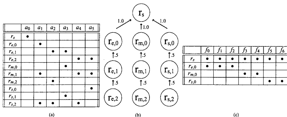
Fig. 8 All security associations and derived mappings for the mouse assembly example: (a) Actor-Role (AR) assignment matrix; (b) Weighted DAG representing the Role Hierarchy (RH). The r_e hierarchy is assigned the electrical subsystem, the r_m hierarchy is assigned the mechanical subsystem, and the r_s hierarchy is assigned the shell; (c) Model-Role (MR) assignment matrix.
