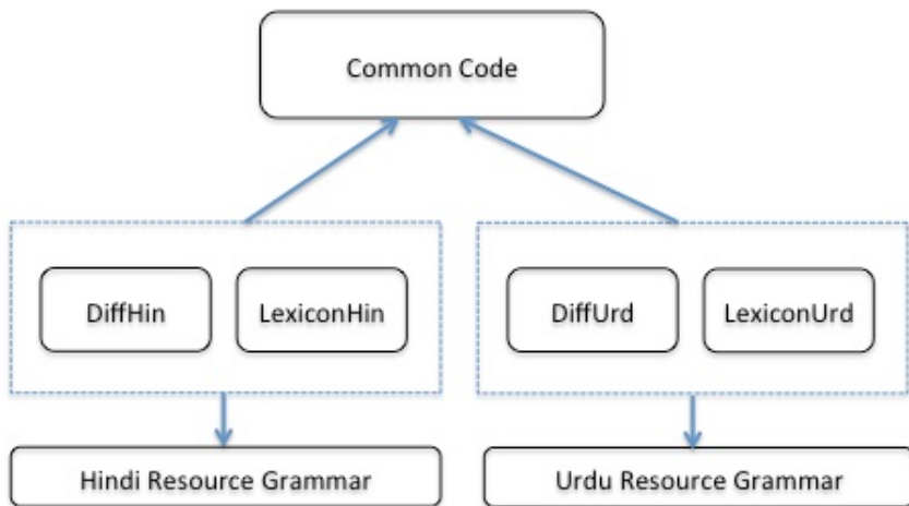
Figure 1: Hindi/Urdu Functor.
