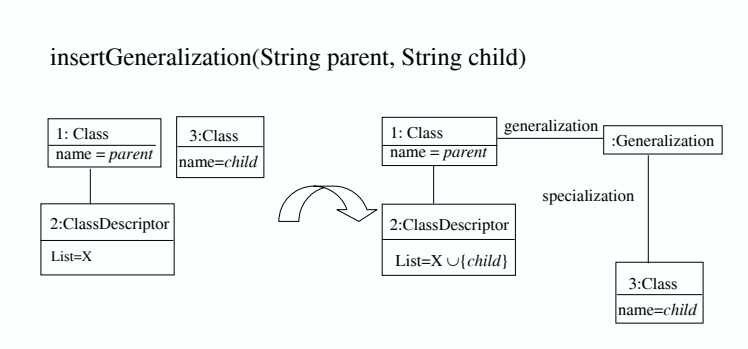
Fig. 3. The rule to insert a generalization relation between two classes.
