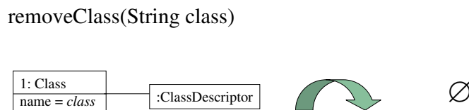
Fig. 5. The rule to remove a class.
