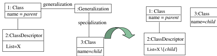
Fig. 4. The rule to remove a generalization relation.
