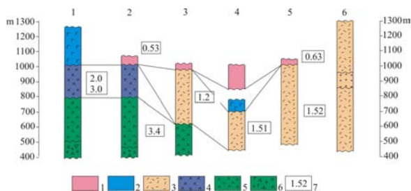
Figure 4. Comparison between the deposits exposed in the walls of Bannaya R. and on slopes of Mount Tolsty Mys. Location of cross-sections (1--6) is shown in Fig. 3: (1) rhyolites, (2) basalts, (3) ignimbrites, crystalline clastic tuffs, (4) dacites, (5) andesites (subvolcanic bodies), (6) tuffs and tuff breccia, (7) K--Ar age, Ma, after Sheimovich and Golovin (2003).
