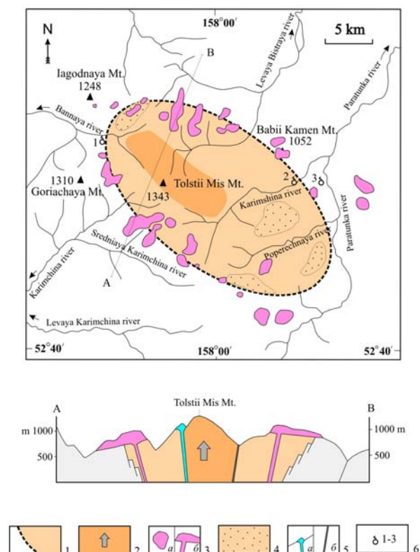
Figure 10. A summary map showing the boundary of Karymshina caldera and its internal structure: (1) boundary of Karymshina caldera and the deposits that fill it (only shown in cross-section), (2) resurgent uplift, (3) rhyolite extrusions and associated lava flows: (a) on map, (b) in cross-section, (4) areas of detected lacustrine deposits (tuff sandstone and tuff aleurolite), (5) small volcanic structures composed of basaltic lavas (a) and ore veins (b) situated at edges of resurgent uplift, (6) thermal springs: (1) Bol'she-Bannaya, (2) Karymshina, (3) Verkhne-Paratunka.
