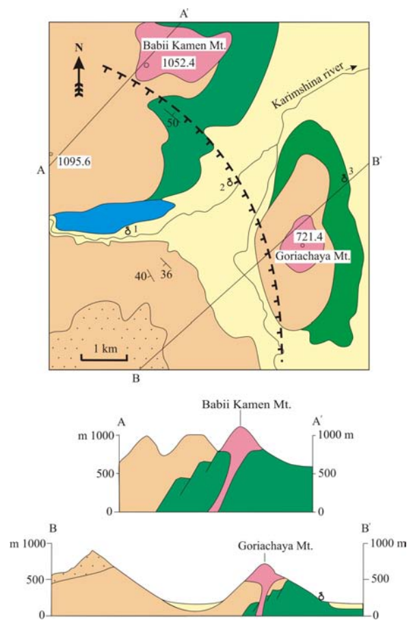
Figure 6. Geological structure and geological cross-sections through the Babii Kamen' area. For notation see Fig. 3. Thermal springs: (1) Verkhne-Karymshina, (2) Karymshina, (3) Verkhne-Paratunka.
