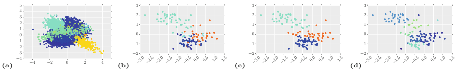
Fig. 3. Example simulated image data using 2D features. (a) Features from all subjects pooled into one set. Colors correspond to true topics, unavailable to the algorithm. (b) Image features for a single subject in a set. (c) Topics recovered by our algorithm (with genetic data) for the same subject based on the whole data set. (d) Topics recovered by k -means clustering applied to the pooled data in (a) (Colour figure online).
