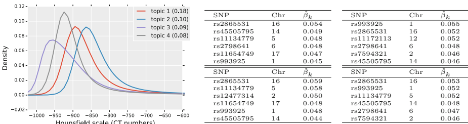
Fig. 4. Four first topics, ranked according to their proportions. Each histogram density is one topic. The values inside of the brackets are the overall proportion computed from the posterior. The tables on the right report the top six SNPs for each topic with their estimated relative weights. We observe that the genetic signatures vary across topics.
