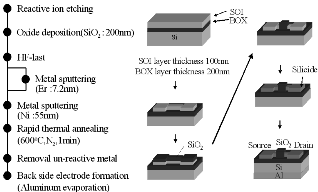
Figure.3 Fabrication process of SOI SB-nMOSFET.
