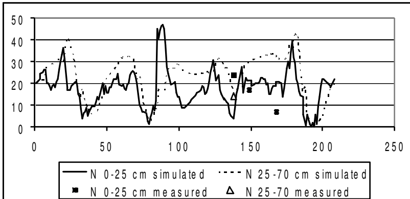
Figure 1: Simulated (lines) and measured (labels) soil inorganic nitrogen. X-axis: week number, 0 = 1 January 2006. Y-axis: \text{kg ha}^{-1} .
