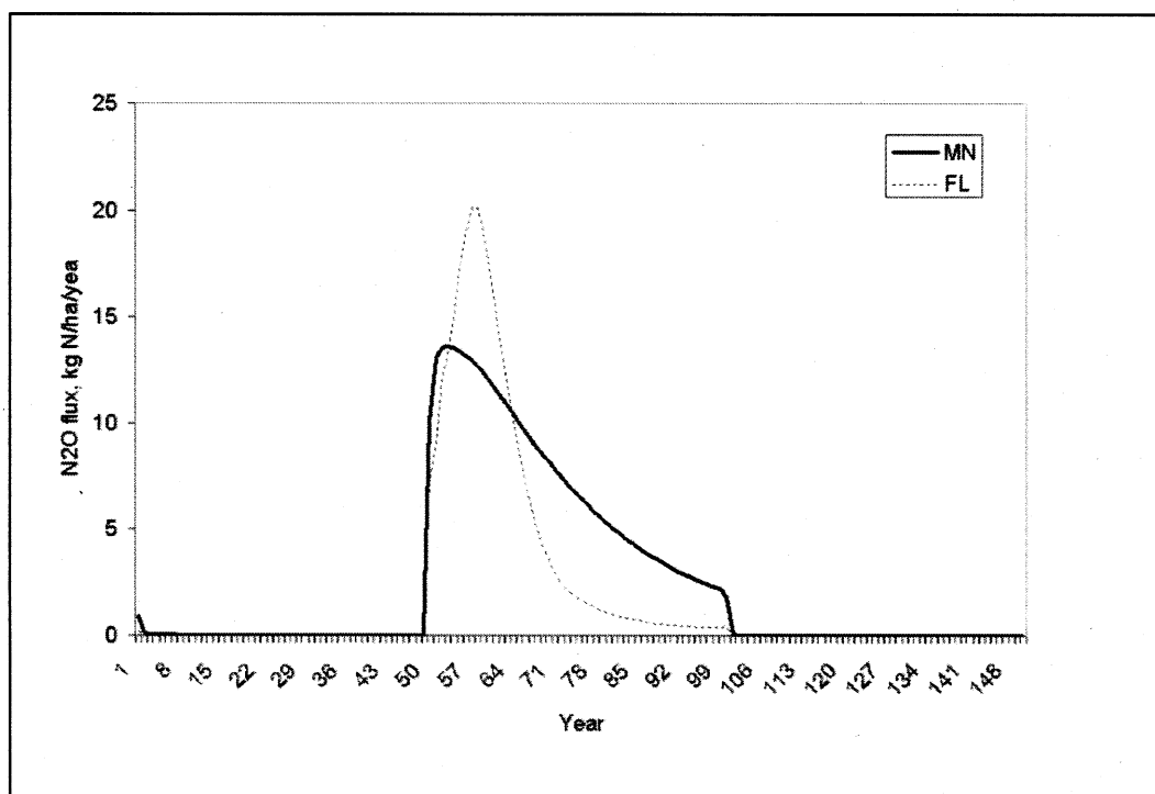
Figure 6. Modeled 150-year \text{N}_2\text{O} emissions from the wetland sites in Minnesota (MN) and Florida (FL). The both sites emitted little \text{N}_2\text{O} under submerged conditions in years 1–50 and 100–150. When the soils were drained after year 50, surges of \text{N}_2\text{O} emissions appeared at the both sites due to the suddenly increased decomposition, nitrification, and denitrification. Driven by the warmer weather, the drainage-induced \text{N}_2\text{O} surges at FL (thin dotted line) were higher but lasted shorter than that at MN (thick line).
