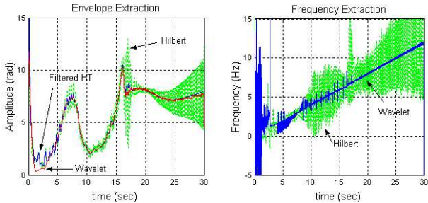
Figure 8. Envelope and instantaneous frequency of input signal
