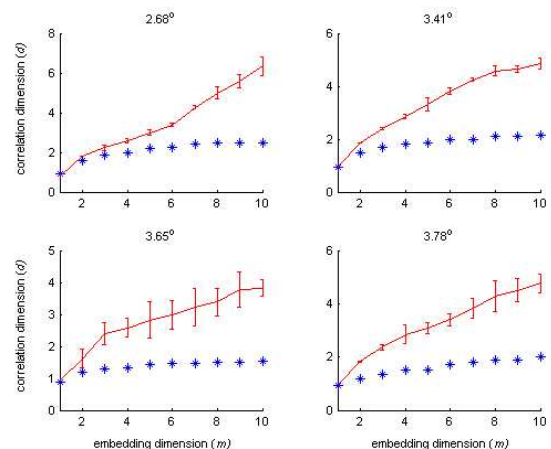
Figure 16. The correlation dimension versus embedding dimension for the original data (excited at excitation level 2.68^\circ , 3.41^\circ , 3.65^\circ and 3.78^\circ ) and for the surrogates. The values of the correlation dimension for the original data and the surrogates differ substantially, and the convergence value of the original data suggests that the underlying dynamics is chaotic.
