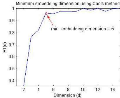
Figure 14. Minimum embedding dimension for CASE 1 system excited by 2.68^\circ input excitation.
