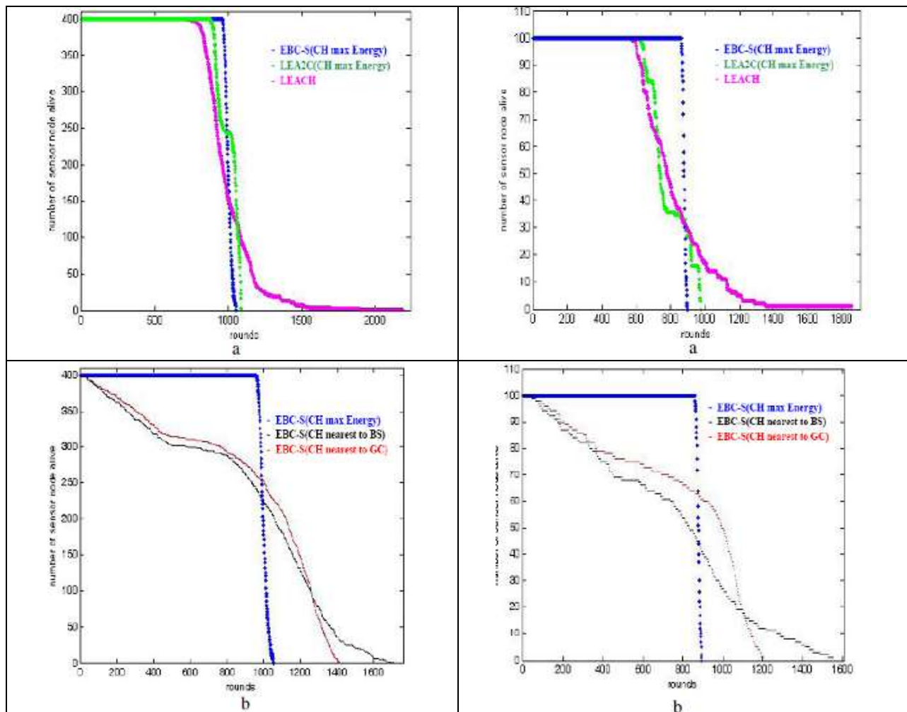
Figure 1: Number of alive nodes VS time (a) comparing in LEACH,LEA2C and EBC-S (proposed algorithm) (b) comparing in EBCS (Proposed algorithm) with different CH criterions (First Scene)
