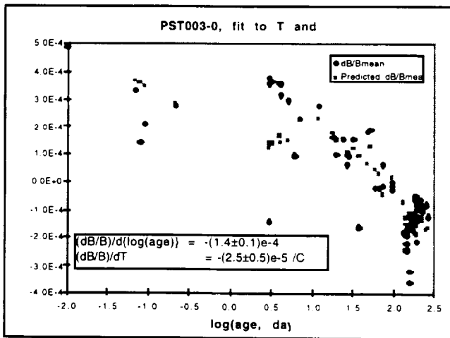
Figure 2. Stability of test magnet #3 as a function of both temperature and time. This fitting accounts for thermal effects due to imperfect temperature compensation.
