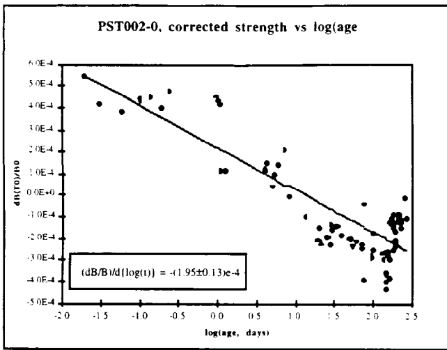
Figure 1. Stability of test magnet #2 as a function of the log of its age. The magnetic strength loss is 0.02% per "decade".
