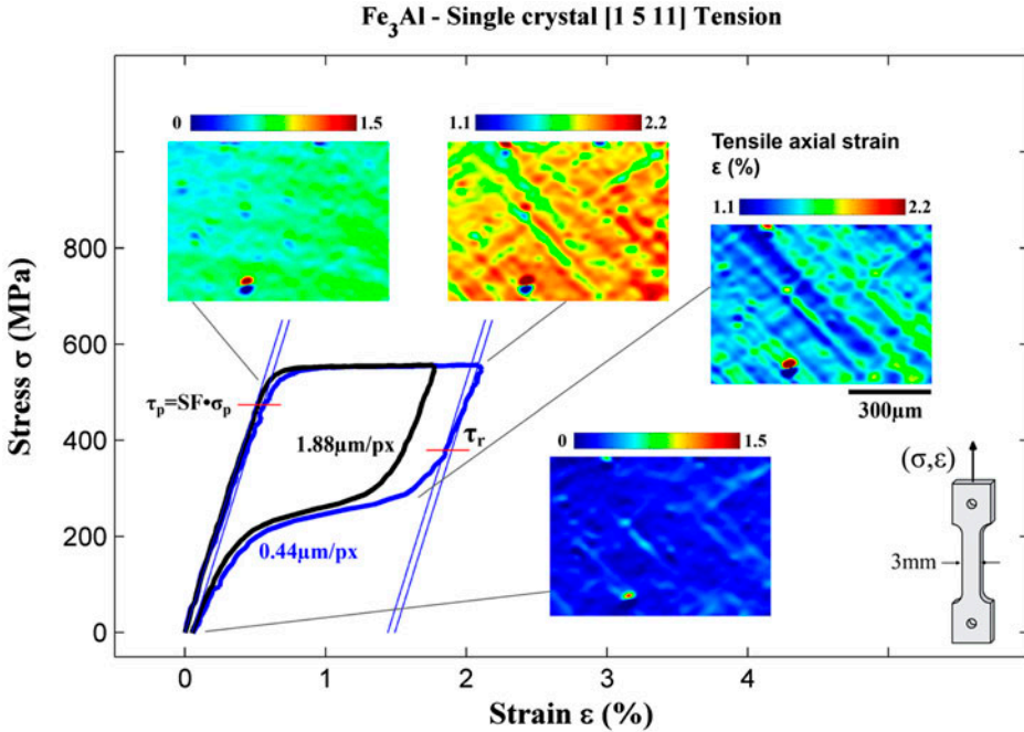
Figure 7. (colour online) Calculation of the critical applied stress \tau_p and the recovery start stress \tau_r from the stress–strain curves for the [1 5 11] crystal orientation in tension. The strain data marked with the black line were obtained averaging the strain fields over a region of 3 \text{ mm} \times 2.25 \text{ mm} , while the strains marked with the blue line were calculated averaging the strain fields over a region of 700 \mu\text{m} \times 525 \mu\text{m} . The applied stress \tau_p and the recovery start stress \tau_r are determined using the blue curve (for more details, see the text).
