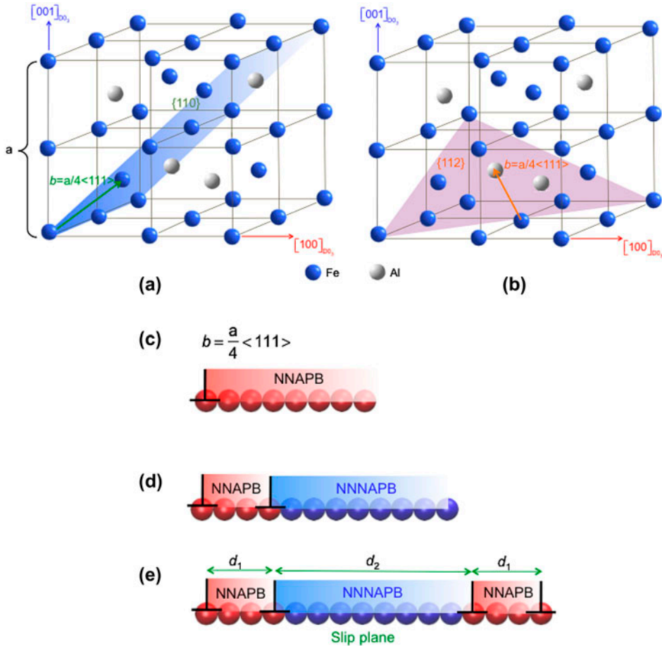
Figure 1. (colour online) D0_3 lattice structure of \text{Fe}_3\text{Al} showing (a) \{110\}\langle 111 \rangle slip system (b) \{112\}\langle 111 \rangle slip system. The length of the arrow gives the magnitude of the partial dislocation with Burgers vector b = a/4\langle 111 \rangle (c) Mode I dislocation configuration, where uncoupled a/4\langle 111 \rangle superpartials leave behind NNAPB ('a' is the lattice constant) (d) Mode II dislocation configuration where paired superpartials leave behind NNNAPB (e) Mode III dislocation configuration where a\langle 111 \rangle superdislocation dissociates into four a/4\langle 111 \rangle dislocations.
