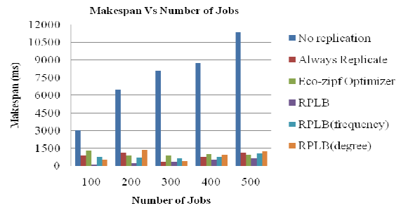
Figure 4. Makespan using various data replication algorithms.
