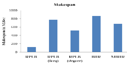
Figure 7. Makespan for executing 100 jobs.
