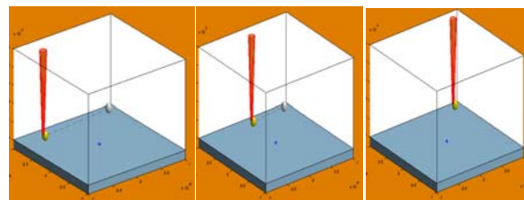
Fig.11 Display of user interface of 3 to 4 stage in which, after touching the particle, probe's tip pushes it toward its destination (white globe).
