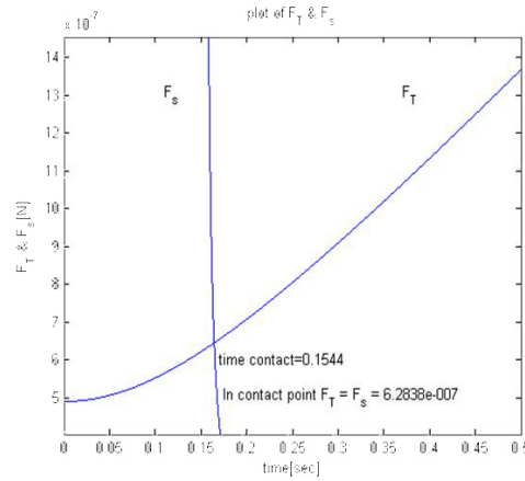
Fig.14 Force diagrams of nano manipulation F_T, F_S^* based on rectangular cantilever of AFM
