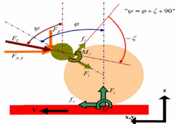
Fig. 5 Schematic diagrams of interaction forces and the resultant deformations between tip/particle and particle/substrate [9]
