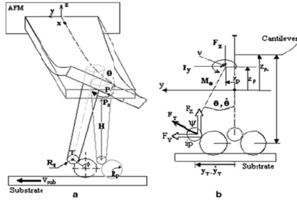
Fig. 4 Schematic diagrams of nanoparticle pushing: a Cantilever deformation in lateral motion. b Free-body diagram of the particle displacement [9].
