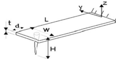
Fig. 3 Schematic diagram of RC AFM probe with off-end tip with distance, d , from free end of cantilever [9]
