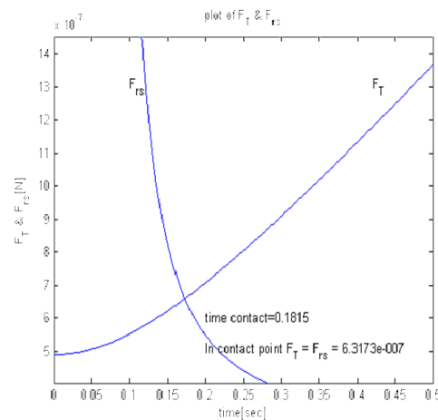
Fig.15 Force diagrams of nano manipulation F_T, F_r^* based on rectangular cantilever of AFM
