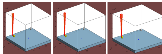
Fig. 10 Display of 2 to 3 stage of the nanomanipulation in which the tip of the probe moves toward the particle.
