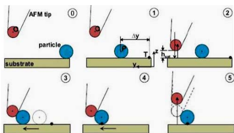
Fig. 6 Strategy of pushing the nano particle in contact mode.[10]
