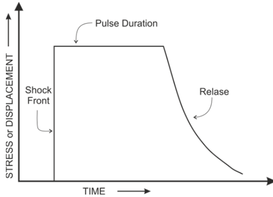
Figure 1. (a) idealized and (b) generic realistic shock wave profile (from Meyers [10]).
