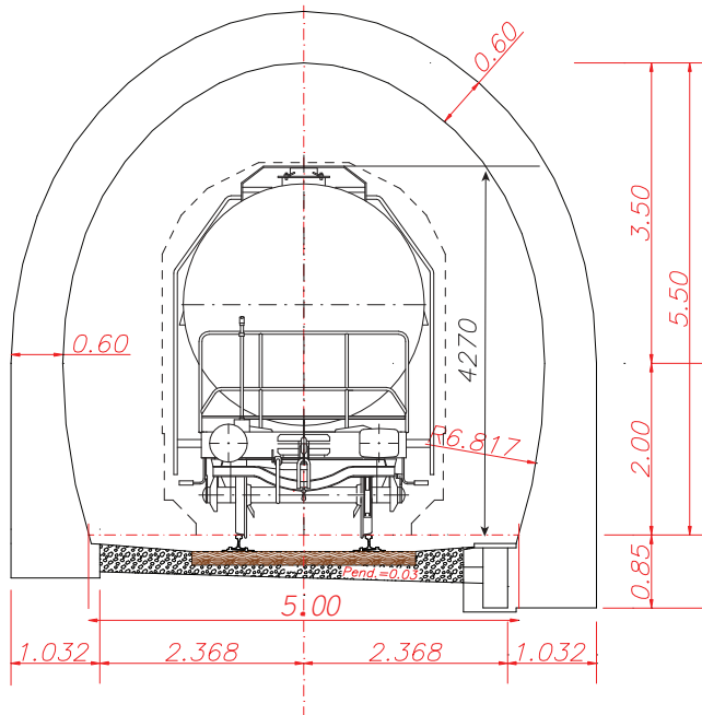
Figure 8. Rail tunnel section.
