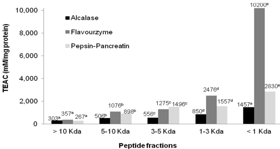
Figure 2. Antioxidant activity of peptide fractions obtained by ultrafiltration from V. unguiculata protein hydrolysates.
