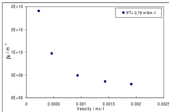
Fig. 8—Variation of \beta_g with gas superficial velocity at S_c=0.40 PV IFT= 0.78 \text{ mNm}^{-1} , Berea core
