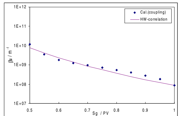
Fig. 9— Comparison of \beta_g as calculated with coupling and predicted by in-house correlation at Sw_i=0.0\% and IFT of 0.78 \text{ mN/m} , Clashach core
