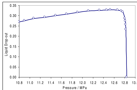
Fig. 1—Liquid drop-out of binary methane n-butane Gas condensate fluid
