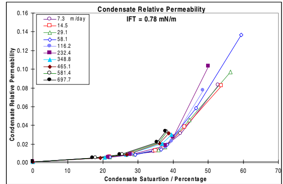
Fig. 3—Clashach core condensate relative permeability
