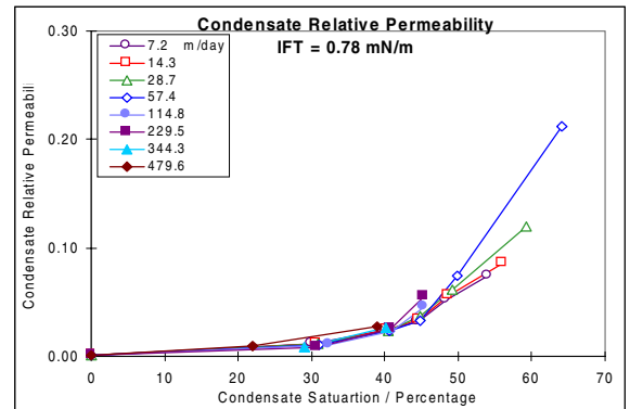
Fig. 5—Berea core condensate relative permeability
