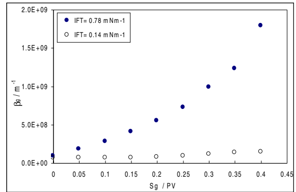
Fig. 7—Variation of \beta_g with Condensate Saturation and IFT
