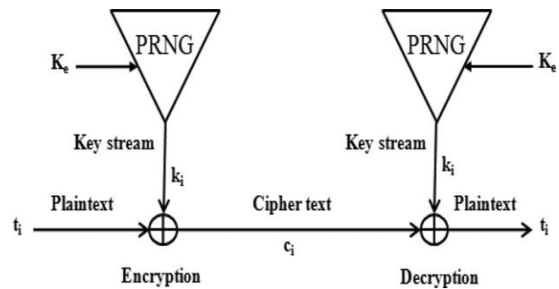
Fig. 2. Encryption/Decryption Process of a Stream Cipher Algorithm
