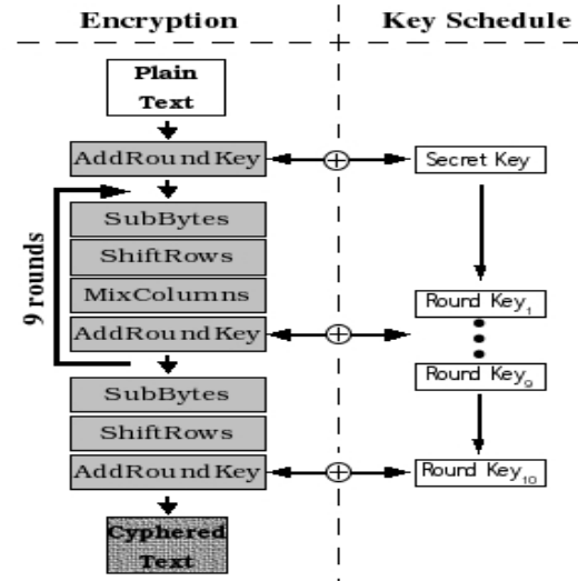
Fig. 5.General Structure of AES Algorithm
