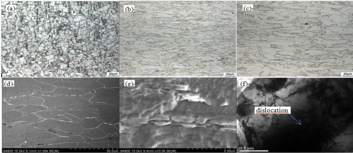
Fig. 3: Microstructure of cold low carbon steel in different deformation, Metallograph: (a) initial microstructure, (b) e = 39.27\% , (c) e = 75.4\% , Microstructure for SEM: (d) e = 28.56\% , (e) e = 75.4\% , Microstructure for TEM: (f) e = 75.4\%
