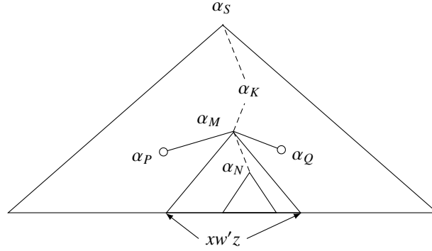
Figure 2: Incremental evaluation of semantic attributes
