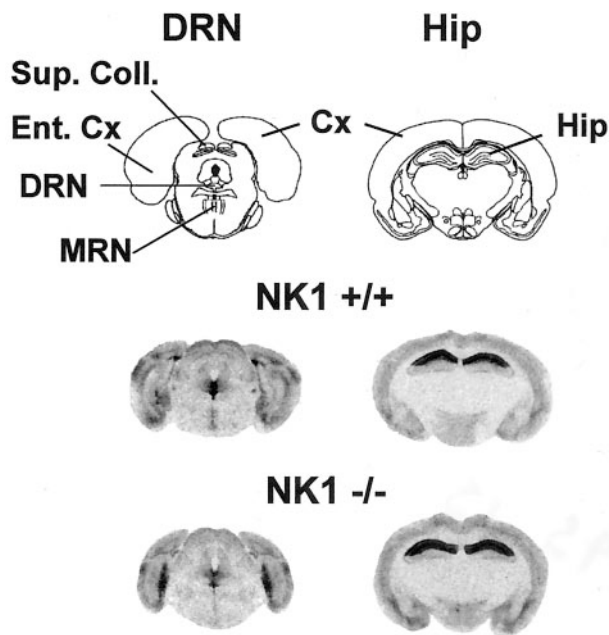
Figure 1. Representative autoradiographic labeling of 5-HT 1A receptors by [ 3 H]WAY 100635 in brain sections from NK1 -/- mutants compared with NK1 +/+ wild-type mice. Coronal sections (20 μm) at the level of the DRN and the hippocampus were labeled with 1 nM [ 3 H]WAY 100635. Similar autoradiograms were obtained from three to five mice per group. Cx, Cerebral cortex; DRN, dorsal raphe nucleus; Ent. Cx, entorhinal cortex; Hip, hippocampus; MRN, median raphe nucleus; Sup. Coll., superior colliculi.
