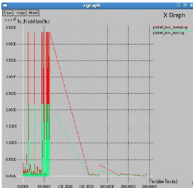
Figure 7: Variation of number of packet loss with simulation time
