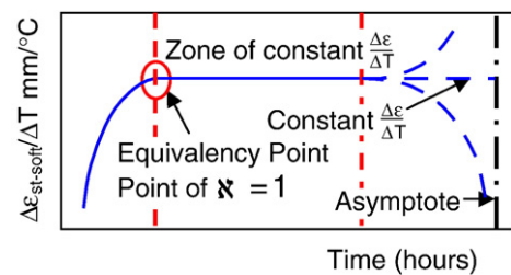
Fig. 5. Predicted shape of the \frac{\Delta \epsilon_{st-soft}}{\Delta T} curve.
