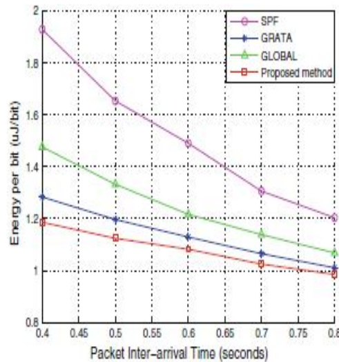
Fig 4: Average energy consumption
