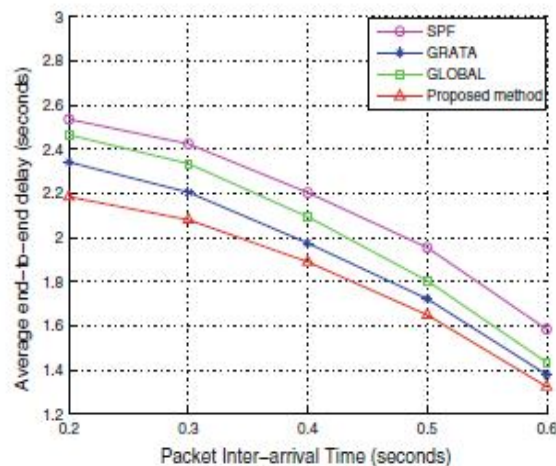
Fig 2: Average end to end delay
