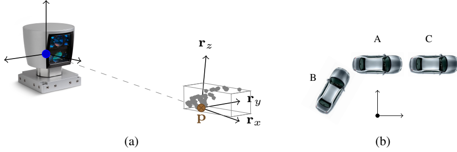
Fig. 3. (a) Illustration of (3). For each vehicle point \mathbf{p} , we define a specific coordinate system which is centered at \mathbf{p} . The x axis ( \mathbf{r}_x ) of the coordinate system is along with the ray from Velodyne origin to \mathbf{p} (dashed line). (b) An example illustration about the rotation invariance when observing a vehicle. Vehicle A and B have same appearance. See (3) in Section III-C for details.
