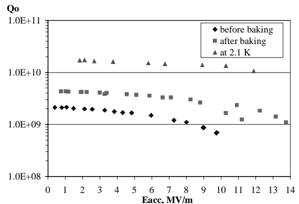
Figure 2. Q vs. E_{acc} plot for spare cavity tested before and after 140°C, 48 hr bake.
