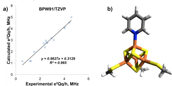
Figure 2. (a) Graph showing correlation between experimental and computed e^2qQ/h values for a series of model systems; (b) Model used in quantum mechanical calculation of the 14 N e^2qQ/h value for IspH+7 complex.
