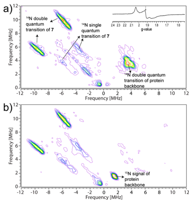
Figure 1. HYSORE spectra of A. aeolicus IspH + pyridine inhibitor 7. (a) HYSORE spectra of unlabeled A. aeolicus IspH + 7. The inset shows the CW-EPR spectrum, and the arrow indicates the magnetic field position for collecting the HYSORE data. (b) HYSORE spectra of ^{15}\text{N} -labeled A. aeolicus IspH + 7. Microwave frequency = 9.66 GHz (a), 9.68 GHz (b); magnetic field was set at g_2 = 1.921 ; \tau = 136\text{ns} .
