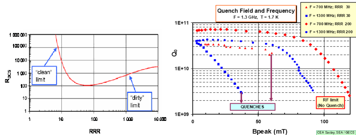
Figure 2: BCS resistance of niobium at 4.2K, and examples of quench field of cavities for different RRR and frequencies (Courtesy of H. Sefa).
