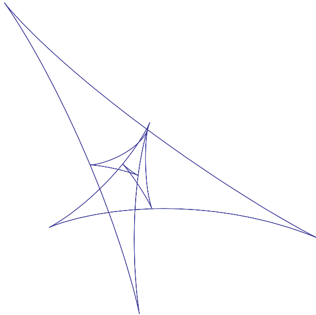
Figure 1. GCS of an oval: CSS with five cusps and the Wigner caustic with three cusps (the medial axis are not shown here).
