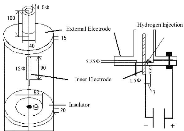
Fig. 1 An illustration of the powder injector
