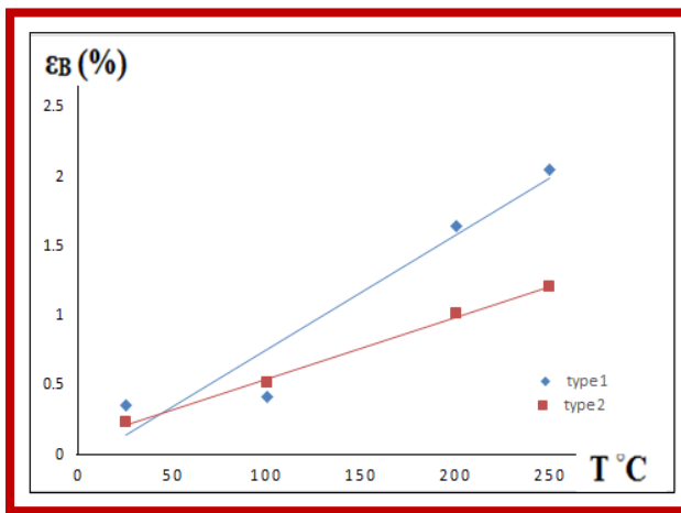
Figure (6) shows strain at breakdown as a function for heat treatment in different temperatures for two types of PTFE.
