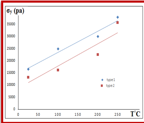
Figure (5) shows stress at yield point as a function for heat treatment in different temperatures for two types of PTFE.
