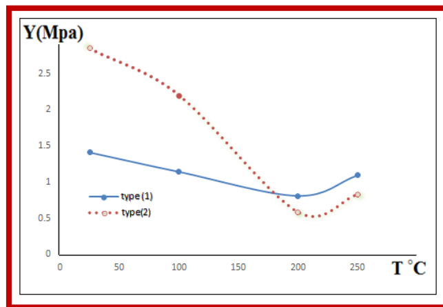
Figure (3) shows Young modulus as a function for heat treatment in different temperatures for two types of PTFE.
