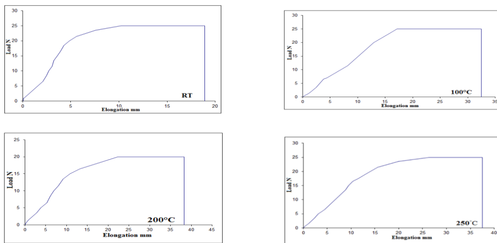
Fig. (2b) Load-Elongation curve for PTFE (type 2) with different temperature for polymer poly (tetrafluoroethylene) PTFE.
