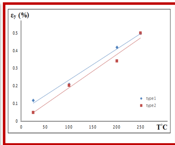
Figure (7) shows strain at yield point as a function for heat treatment in different for two types of PTFE.
