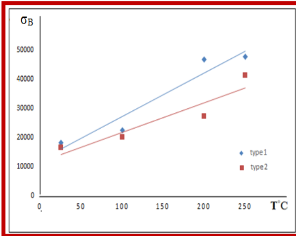
Figure (4) shows stress at break as a function for heat treatment in different temperatures PTFE.
