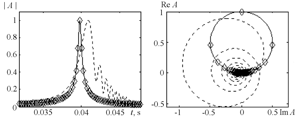
Figure 1. Signals' envelopes (left) and phase diagrams (right) after the band (dashed lines) and correcting (solid lines) filters. Diamonds mark the values of the given transfer function characteristics (16).
