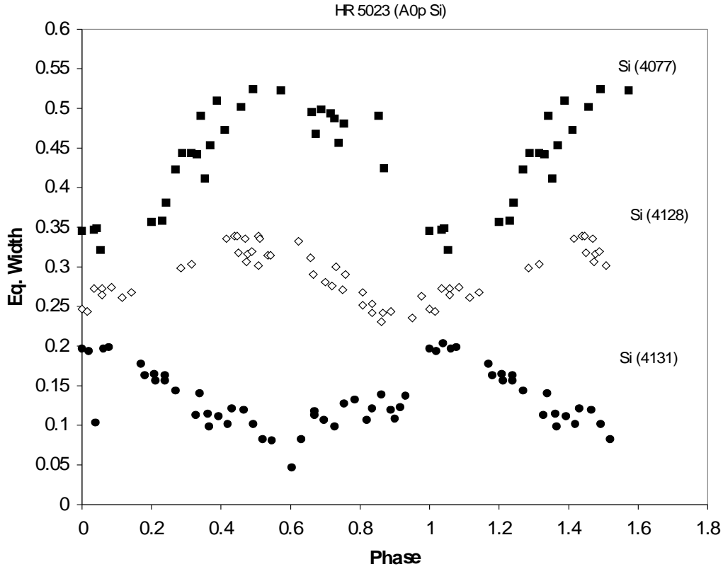
Figure 1. Variations in the spectral lines of Si (4077), Si(4128) and Si(4131) in the Ap star HD 115735 (= HR 5023). The phase is based on the period of 0.88 day and the scale for the equivalent width (in Angstroms) is arbitrary.
