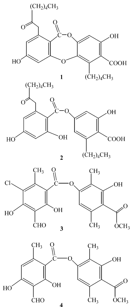
Fig. 1. Chemical structures of physodic acid (1), olivetoric acid (2), chloroatranorin (3), and atranorin (4).
