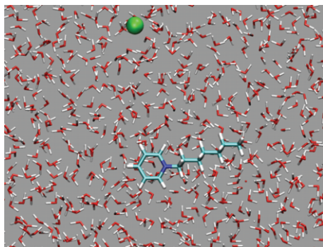
FIGURE 1: Initial configuration of the simulated system. Two counterions were located randomly in the water box. The cation was nonprotonated N-heptyl-pyridine, and the anion was chloride ion (in green).
